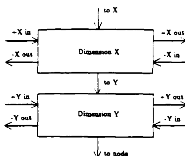
Figure 5: NDF block diagram. An NDF consists of two priority levels each of which is composed of two dimensions.
