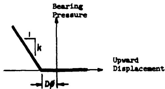
Figure 2 - Spring for Shrinking Soil
