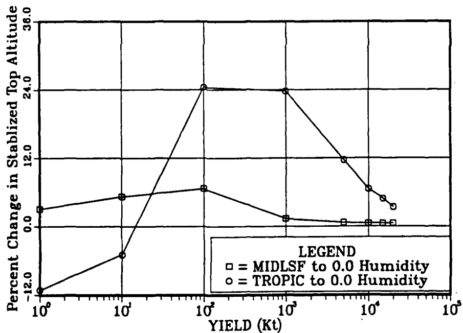
Figure 2. Comparing Stabilized Cloud Top of the MIDLSF and TROPIC Profile Results to the 0.0 Humidity Profile Result - Revised CRM
