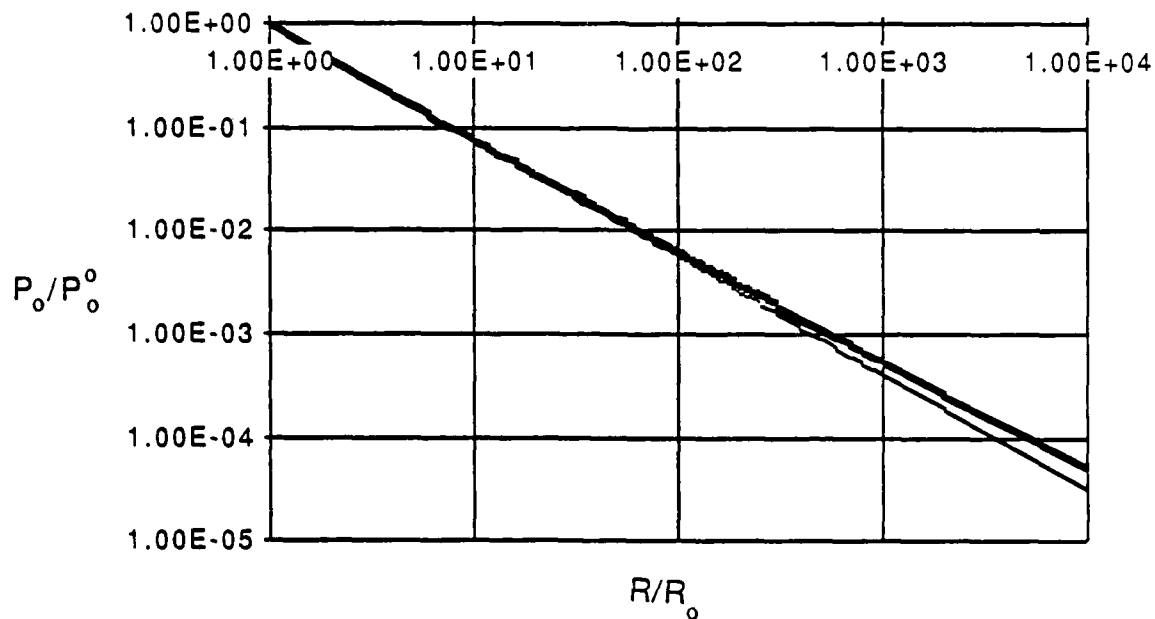
Fig. 10. Empirical and nonlinear pressure-peak decays. Thick line represents nonlinear theory for \tau=0.37 .
