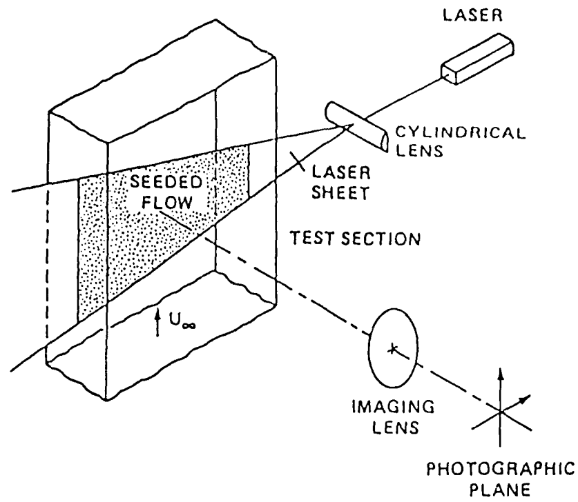
Figure 1. Schematic arrangement for the photographic recording.
