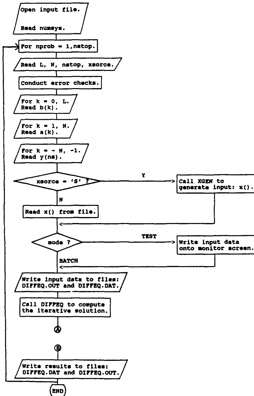
Figure I.2 DIFFEQ.FOR Software Flowchart.
