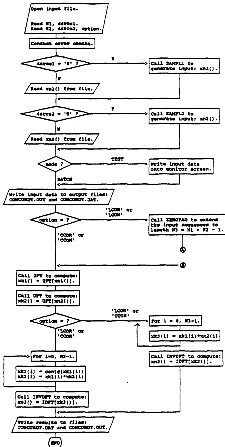
Figure E.5 CONCORDT.FOR Software Flowchart.
