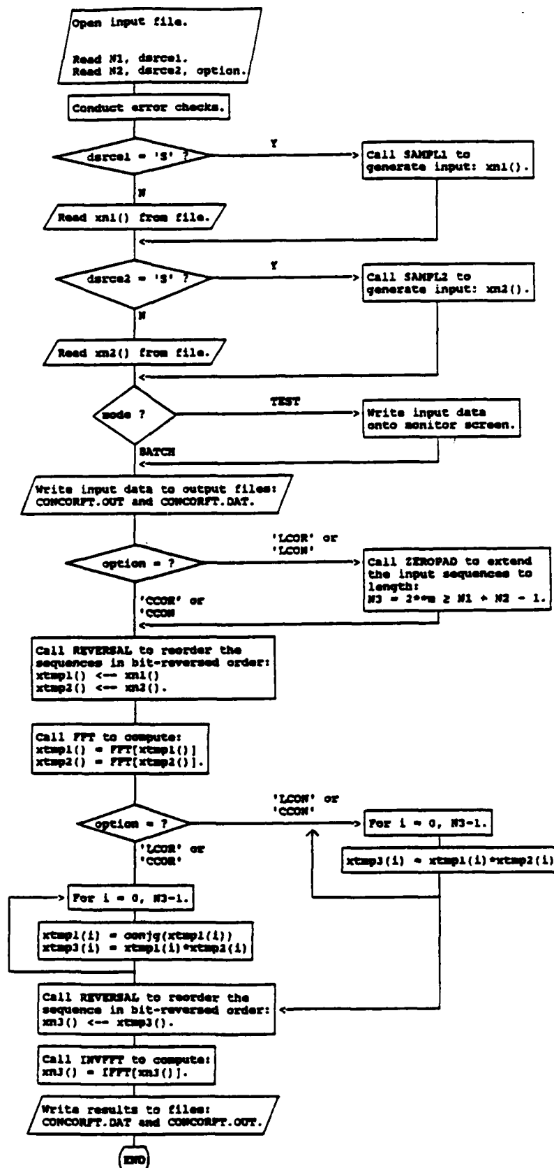
Figure G.5 CONCORFT.FOR Software Flowchart.
