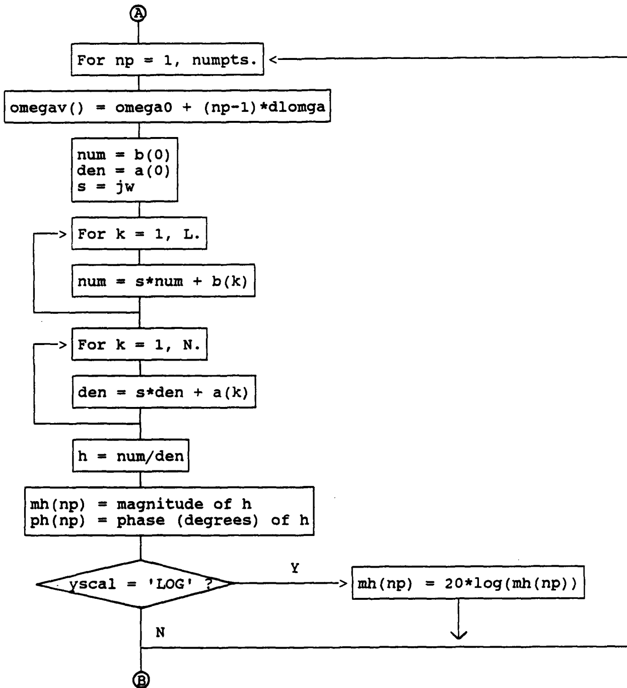
Figure B.4 AFRESP Subroutine Flowchart.
