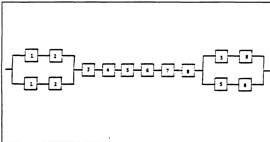
Figure 1. Mixed parallel/series system configuration
