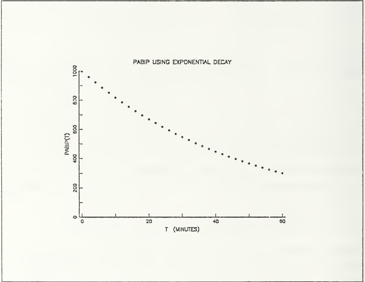
Figure 5. Predicted Basic Inherent Power using Eqn. 4.4
