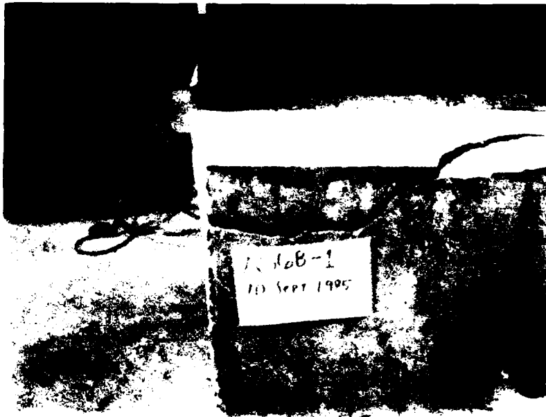
Photo 7. Wall armor test failure, assembly AS6B-1
