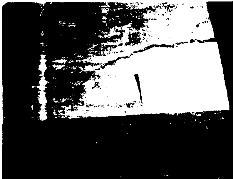
Photo 3. Wall armor test failure, assembly HS6B-1
