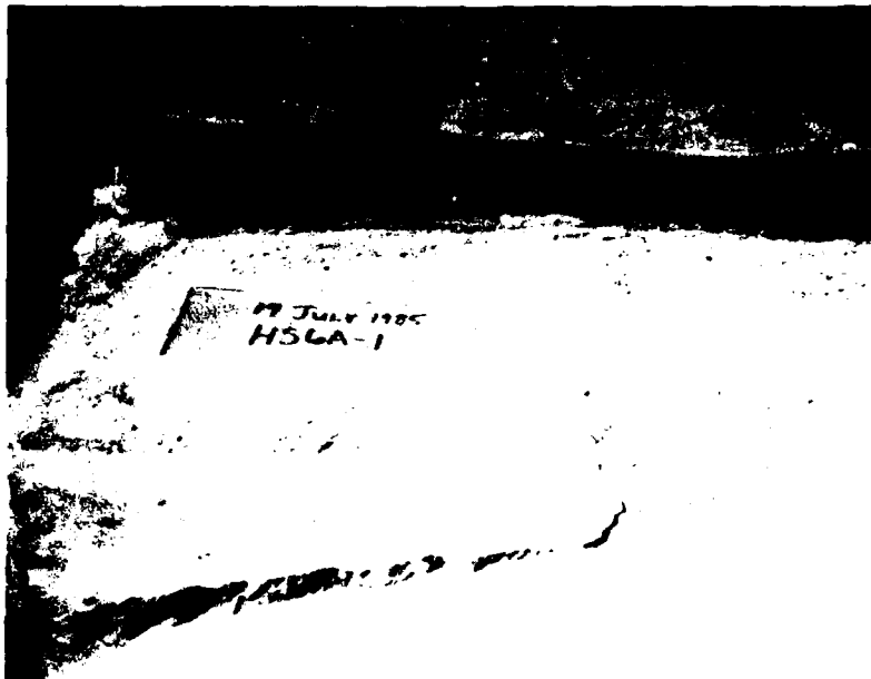
Photo 1. Wall armor test failure, assembly HS6A-1
