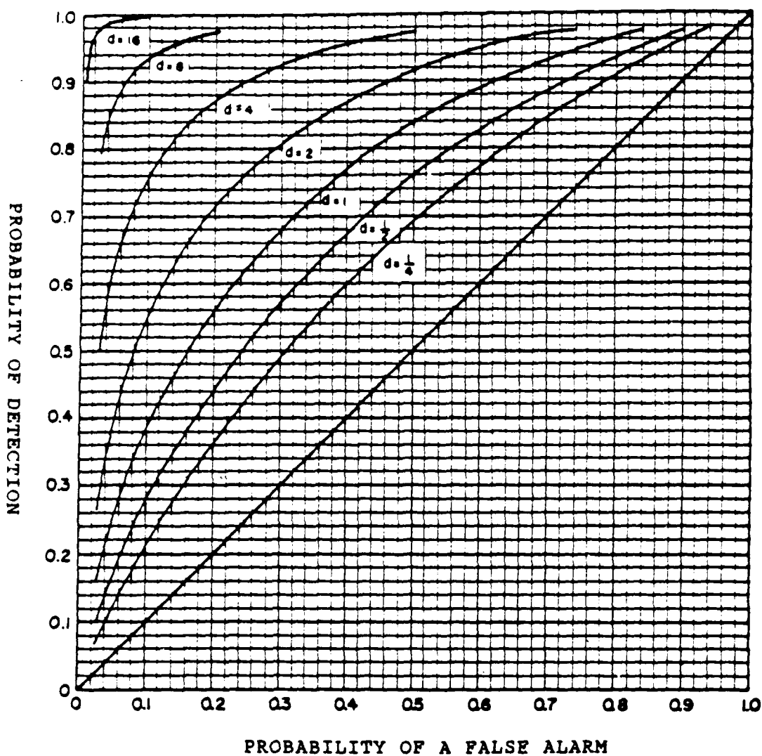
Figure B.3: Receiver Operating Characteristic (ROC) Curve
