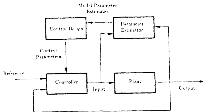
Figure 1: Adaptive Control
