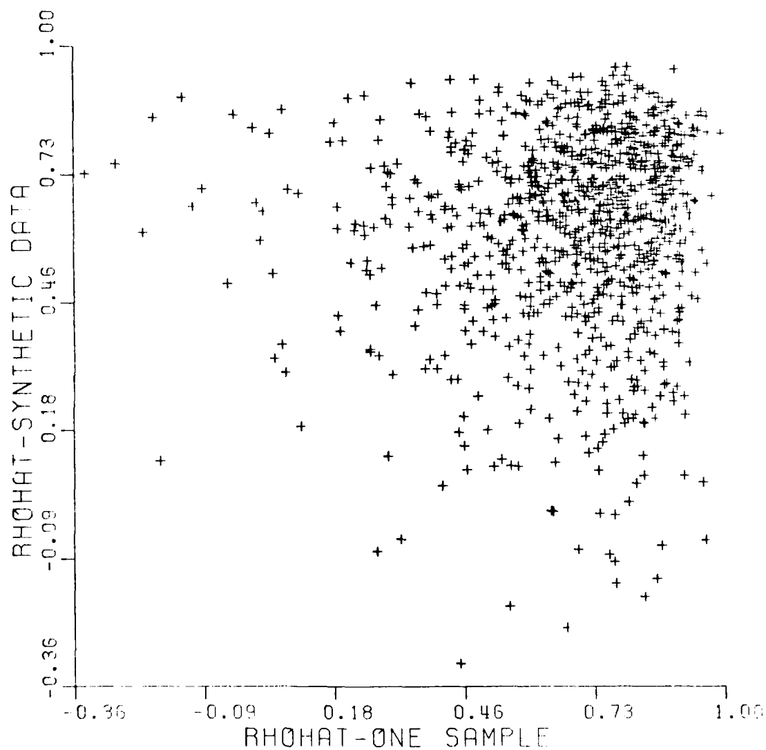
Figure 3.9 Isotonic vs. Nomatching.
