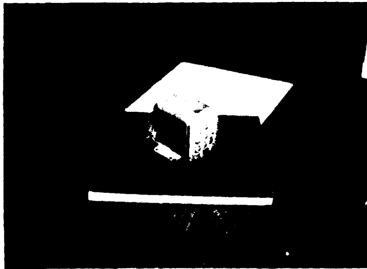
Fig. 11 Relay corrosion.
