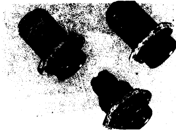
FIGURE 5. GALVANIC CORROSION OF NICKEL PLATED ALUMINUM COAXIAL CONNECTORS
