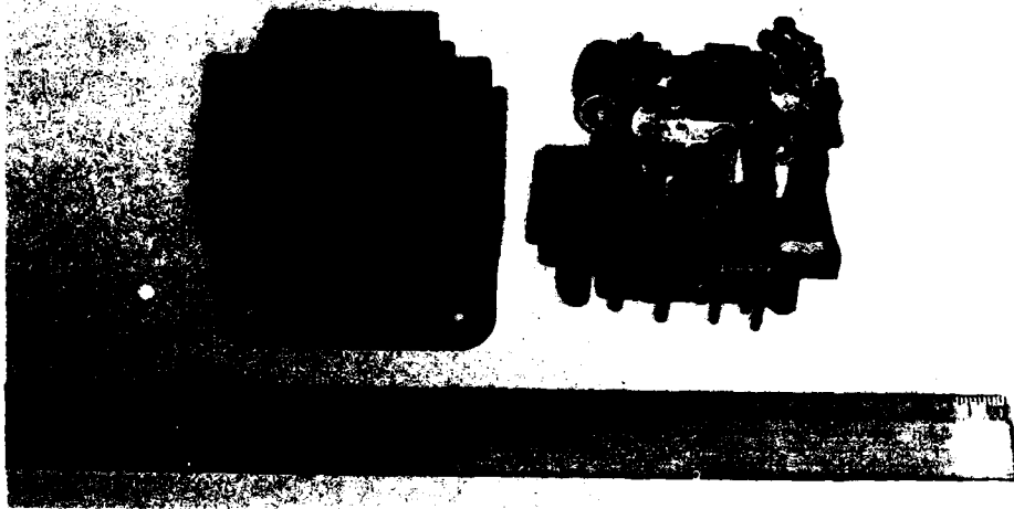
Fig. 15 Relay exhibiting corrosion resulting from "Fresh" water immersion of a Sea King Helicopter.
