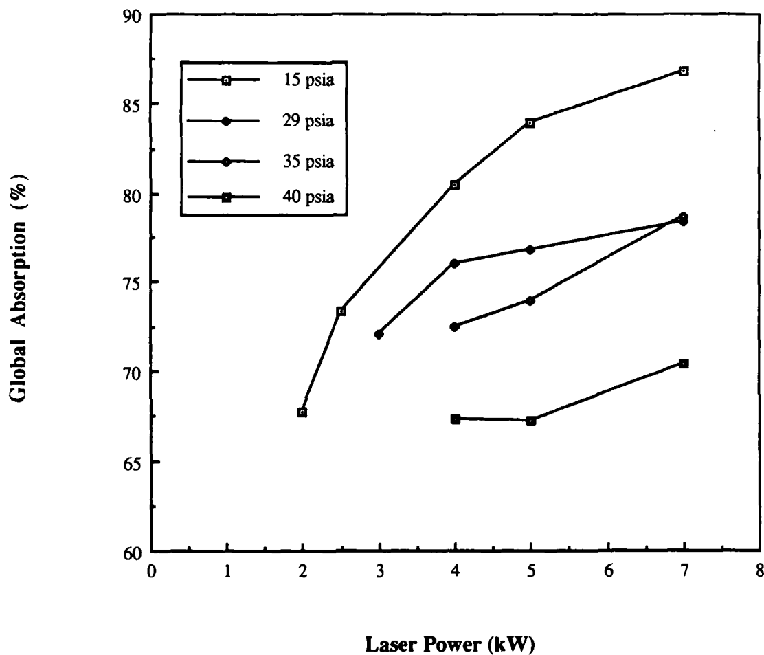
Figure 4.5 Global absorption percentage as a function of input laser power. The mass flux is 8.95 kg/sm 2 in all cases. Results are shown for four different gas pressures.
