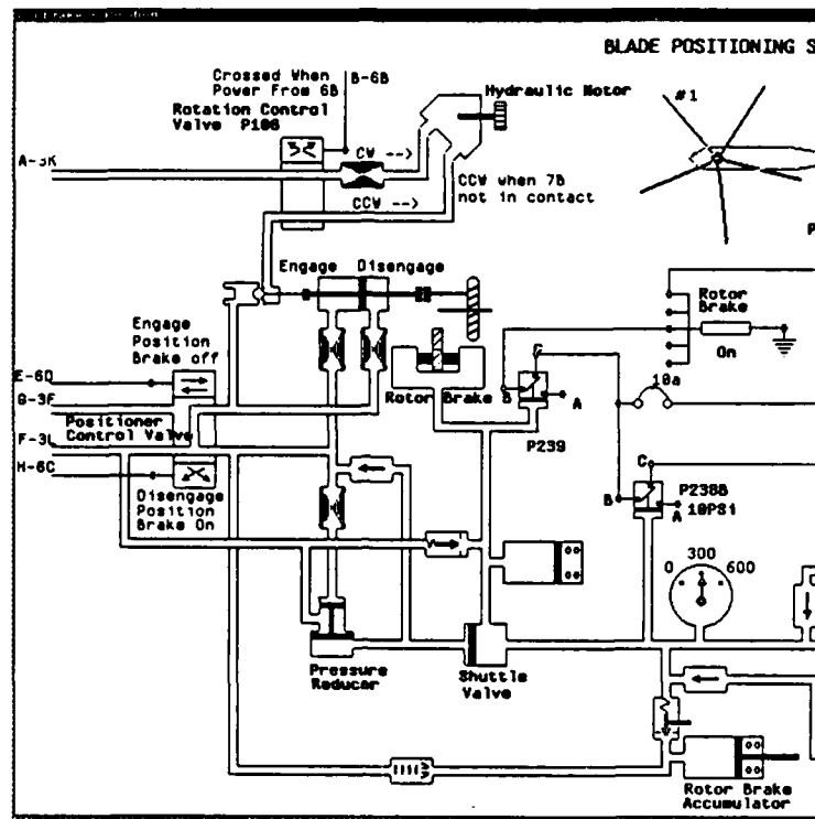
Figure 5. A Scene from the IMTS Bladefold Graphical Simulation
