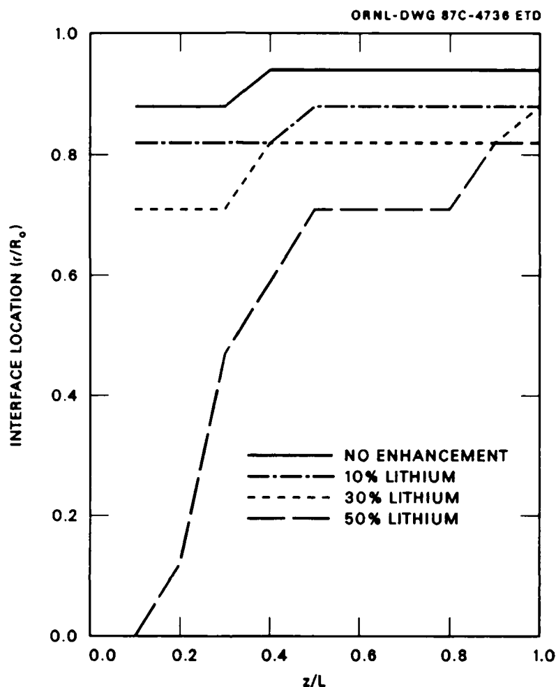
Fig. 4.7. Phase-Change Front Positions for Liquid Lithium Enhancements.
