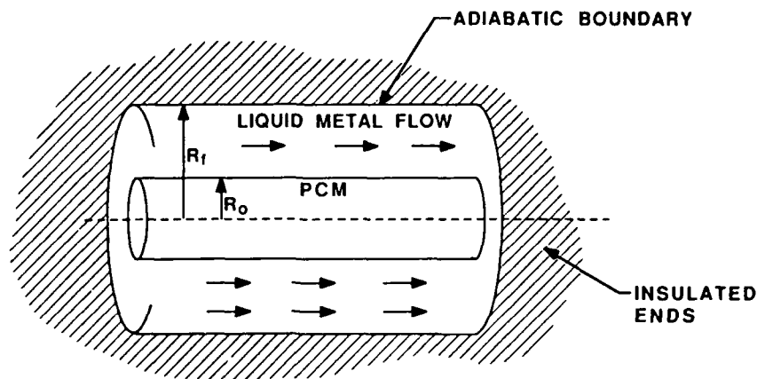
Fig. 1.2. Model Schematic.
