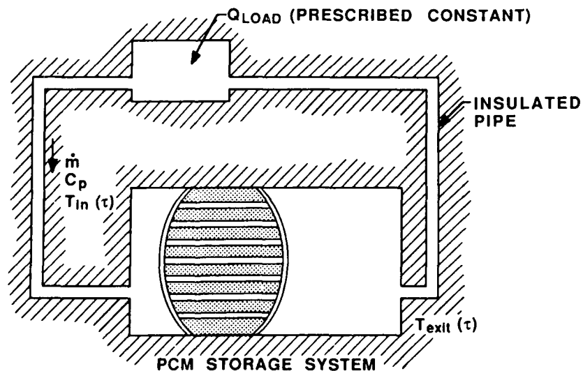
Fig. 1.1. System Schematic.
