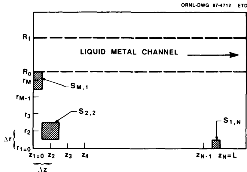
Fig. 3.1. Finite Difference Element Grid.
