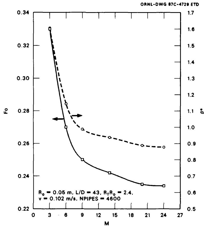
Fig. 3.5. Effect of Element Size on Test Duration ( F_o ) and Energy Storage ( \theta^* ).
