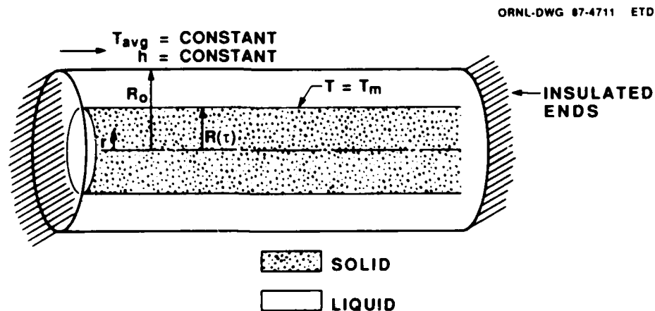
Fig. 2.1. Approximate Model of the PCM Region.
