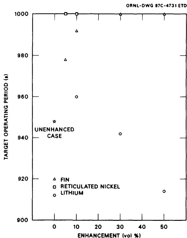
Fig. 4.2. Effect of Enhancements on Test Durations.
