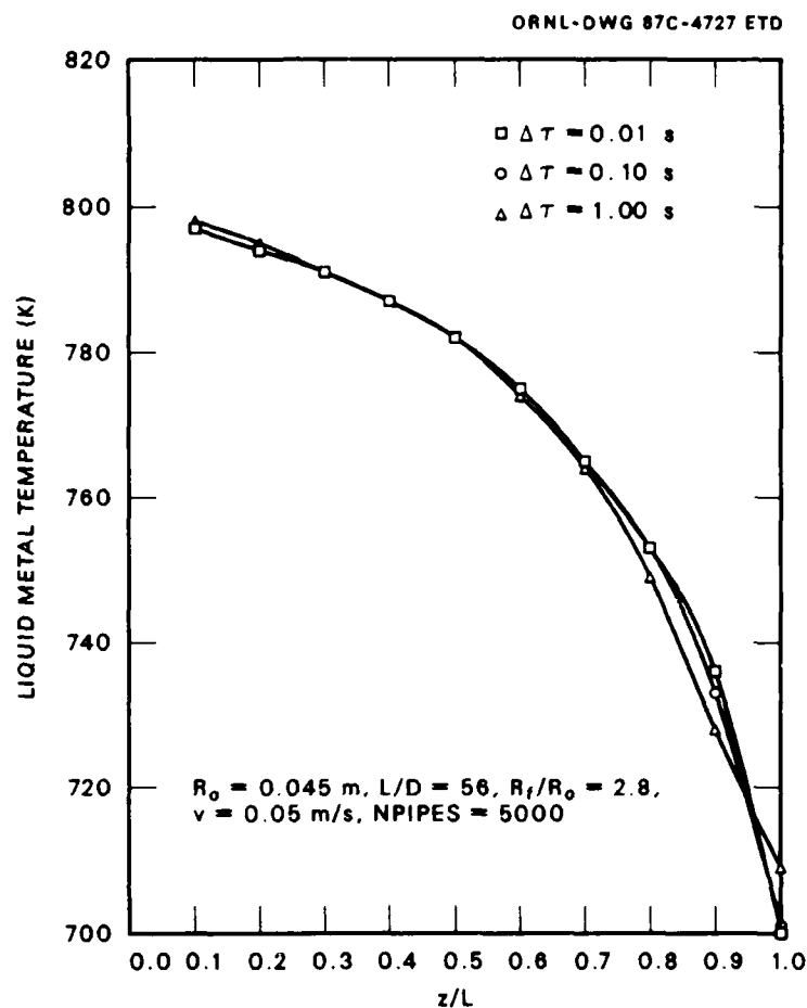
Fig. 3.3. Influence of Time-Step Size on the Stability of the Implicit Solution.
