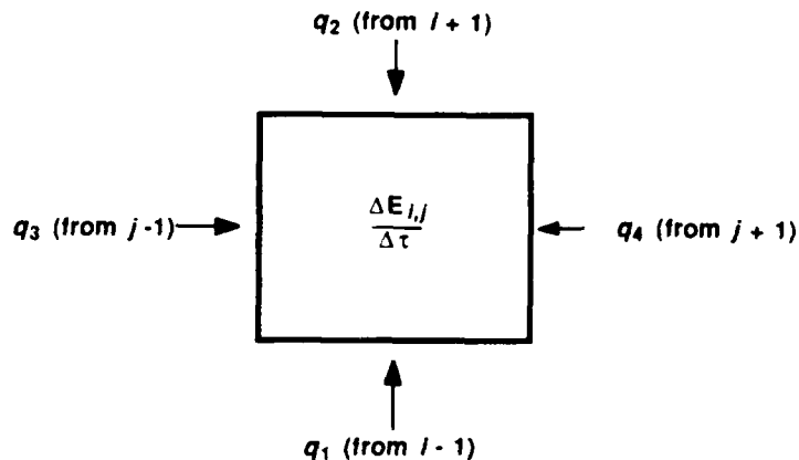
Fig. 3.2. PCM Node Energy Balance.
