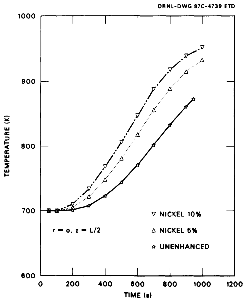
Fig. 4.10. Temperature Response of Central PCM Node for Systems Enhanced With Reticulated Nickel.
