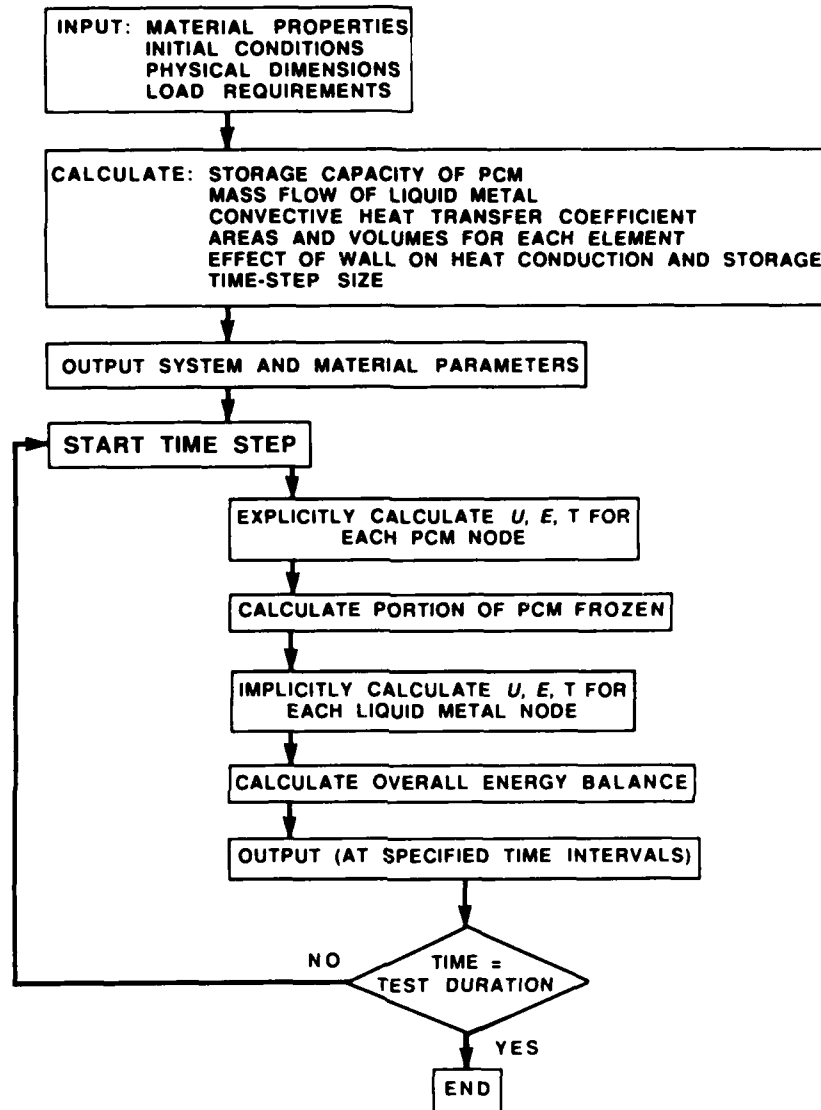
Fig. 3.6. Flow Chart for Finite Difference Computer Code.
