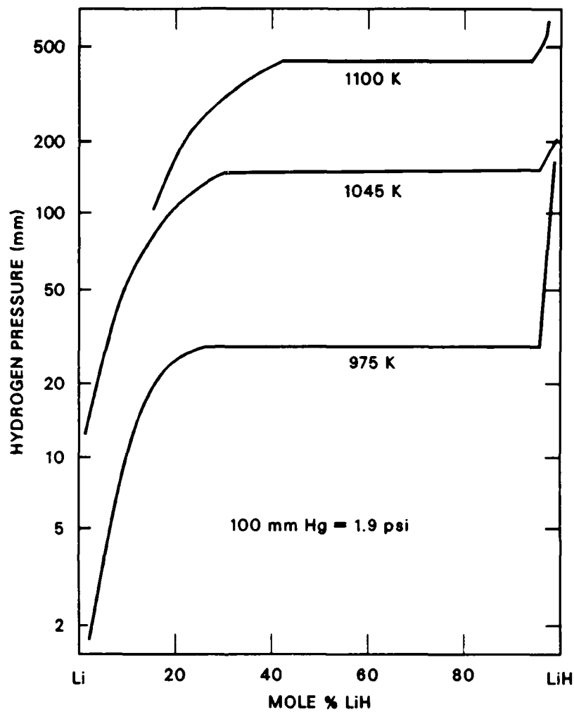
Fig. 3.7. LiH Hydrogen Pressure is Lowered by the Addition of Liquid Lithium.
