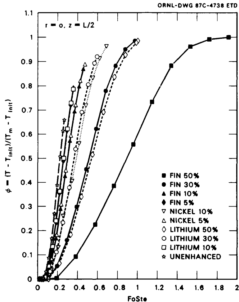
Fig. 4.9. Nondimensional Time Response of Central PCM Node for Enhanced Configurations.
