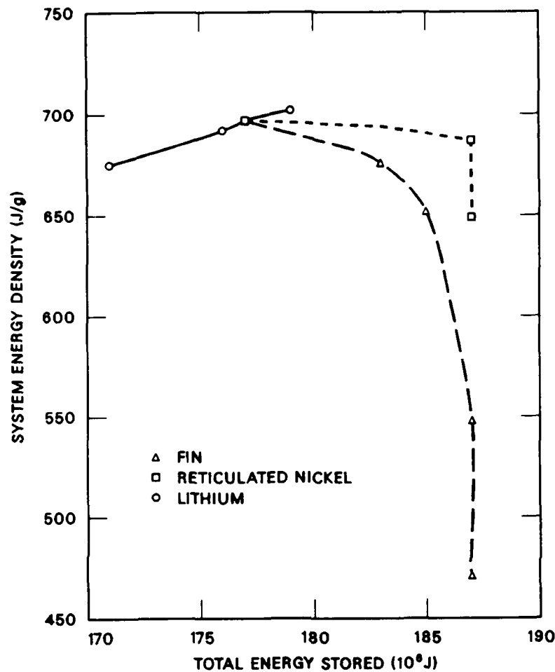
Fig. 4.5. System Energy Density vs Total Energy Stored for Enhanced Systems.
