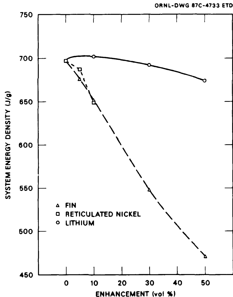
Fig. 4.4. Effect of Enhancements on System Energy Density.
