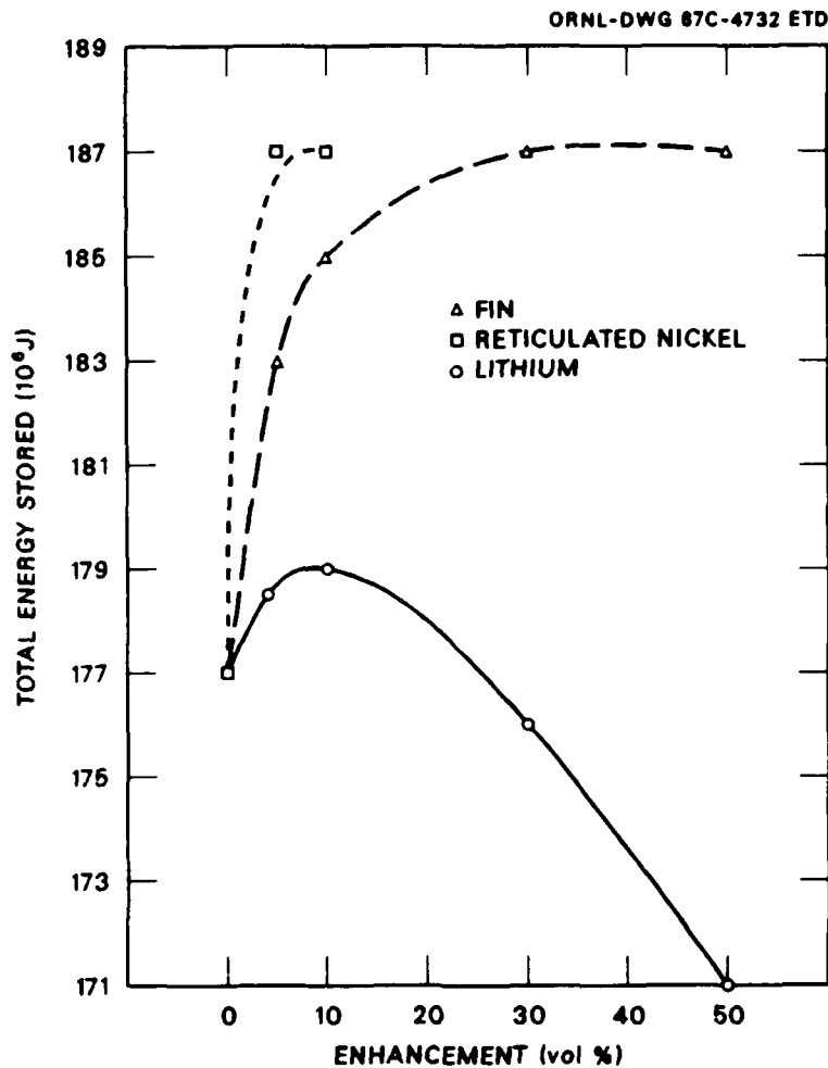
Fig. 4.3. Effect of Enhancements on Total Energy Storage.
