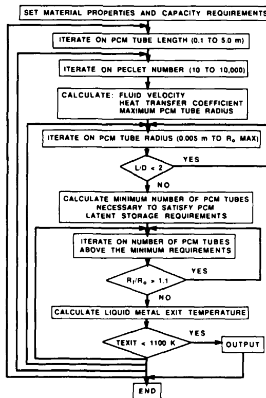
Fig. 2.2. Flow Chart for Approximate Solution Computer Code.
