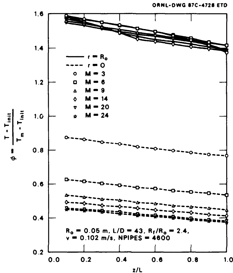
Fig. 3.4. Effect of Element Size on PCM Dimensionless Temperature Profile.
