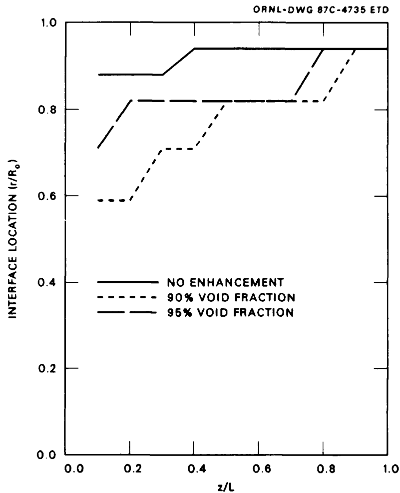
Fig. 4.6. Phase-Change Front Positions for Reticulated Nickel Enhancements.
