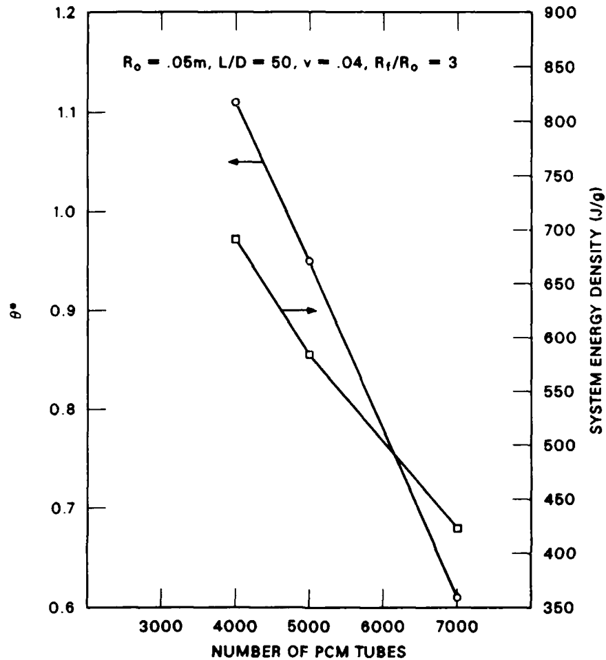
Fig. 4.1. Energy Stored per Tube vs Number of PCM tubes.
