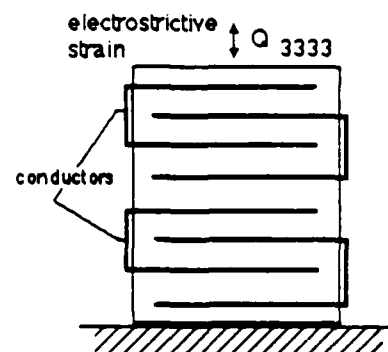
Fig. 5 Multilayer Actuator Configuration
