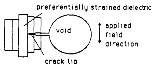
Fig. 8 Enhanced Electrostriction near Crack
