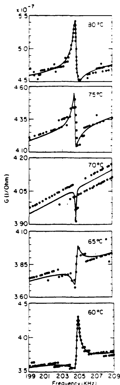
Fig. 6. Plots of conductance ( G ) versus frequency near the temperature where \chi goes through minimum for Sm-modified lead titanate. Dots are experimental points and solid line is a fit to data. Scattering in the data is due to the resolution of the impedance analyzer.
