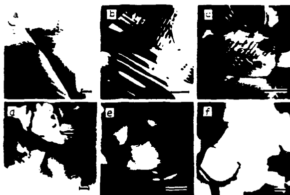
Fig.4 . The variation of the domain configuration of Ca-doped barium titanate ceramics with the increase of the concentration of Ca on the B sites: (a). pure, (b). Ba_{0.95}Ca_{0.05}TiO_3 , (c). Ba_{0.95}Ti_{0.98}Ca_{0.07}O_{2.98} , (d). Ba_{0.95}Ti_{0.97}Ca_{0.08}O_{2.97} , (e). and (f). Ba_{0.95}Ti_{0.96}Ca_{0.09}O_{2.96} . In the pure and slightly doped ceramics, the domains can be easily seen because of their larger size. With increasing Ca concentration on the B site, the domains become vanishingly small. The observed domain sizes vary from 0.3 \mu m to 0.06 \mu m . The scale bar is 0.5 \mu m in every picture.
