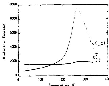
Figure 4. Dielectric constant ( \epsilon_{33}^T and \epsilon_{\perp c}^T ) vs. temperature for orthorhombic \text{Pb}_{0.60}\text{Ba}_{0.40}\text{Nb}_2\text{O}_6 measured at a frequency of 10 kHz.
