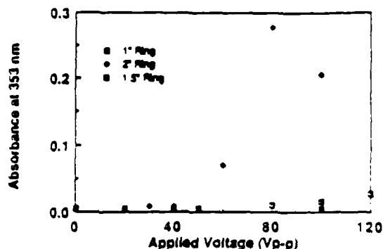
Figure 4. Production of Iodide Trimer at Varying Voltages for Ring Transducers.
