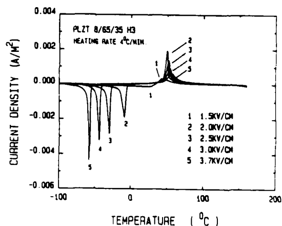
Fig. 7. Typical curves of temperature dependence of current density under different bias field of 8/65/35 PLZT ceramics.
