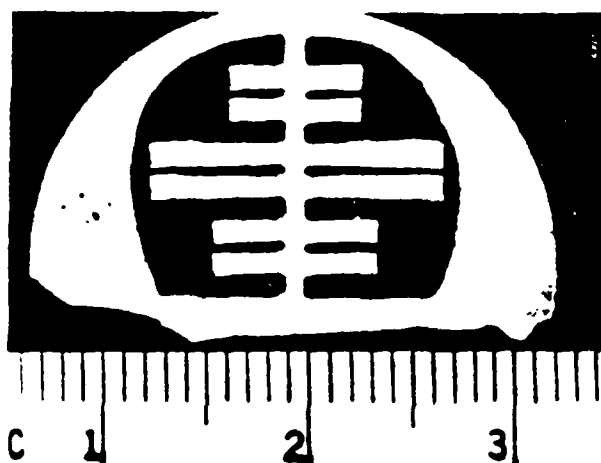
Fig. 4 Piezoelectric Resonator (Numbered divisions in cm)
