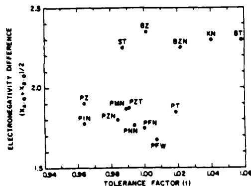
Figure 2. Plot of electronegativity difference vs. tolerance factor.
