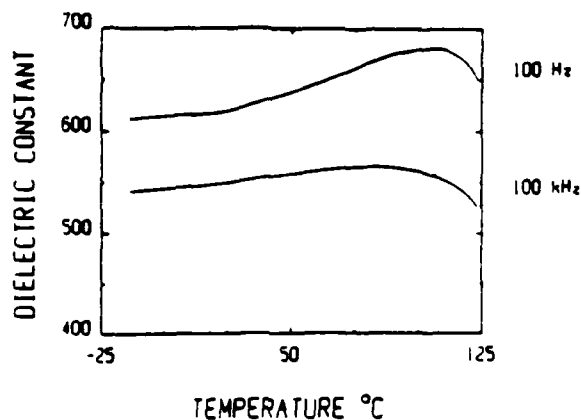
4a. Dielectric constant vs. temperature at 100 Hz and 100kHz.
