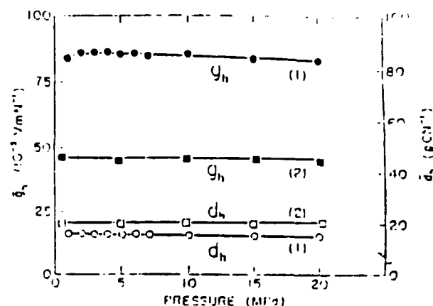
Fig. 2. Variation of \bar{g}_h and \bar{d}_h as a function of pressure for (1) \text{PbTiO}_3 and (2) \text{Pb}_{0.5}\text{Bi}_{0.5}\text{Ti}_{0.5}\text{Fe}_{0.5}\text{O}_3 composites prepared from \text{PbTiO}_3 and BF-PT, respectively.
