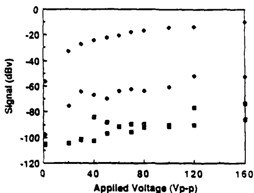
Figure 3B. 1.5" Ring.
