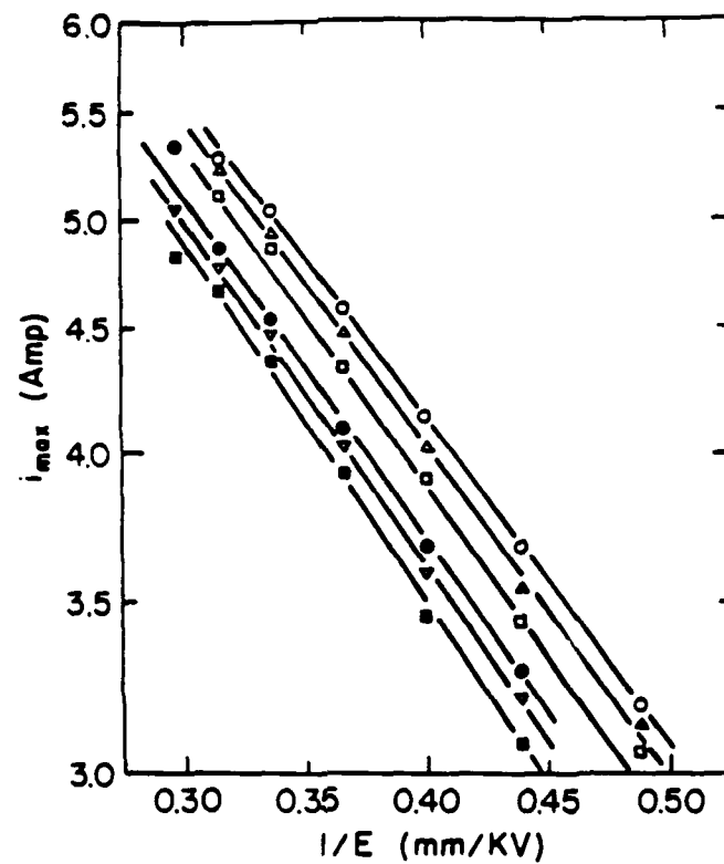
Figure 7 Applied field dependence of peak switching current under various hydrostatic pressures in coarse grain PZT ceramics.
