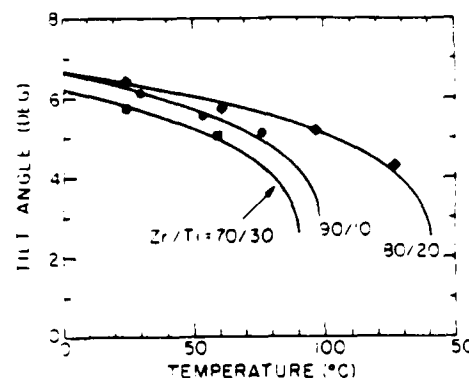
Figure 6. The spontaneous tilt angle plotted versus temperature.
