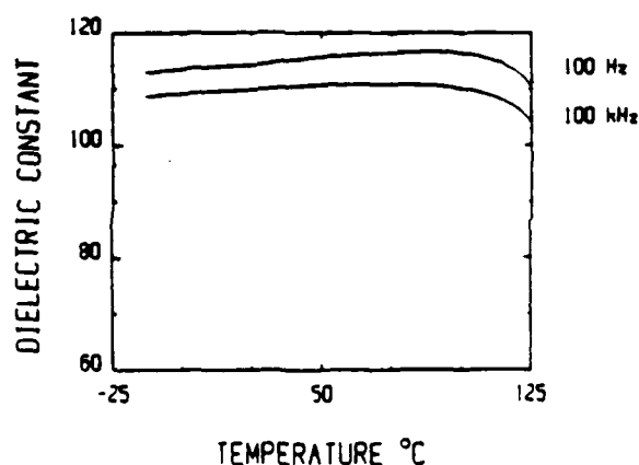
5a. Dielectric constant vs. temperature at 100 Hz and 100kHz.
