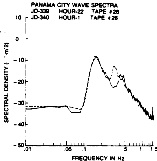
Fig. 18 — Change in spectral density between first and last hours of run 26.
