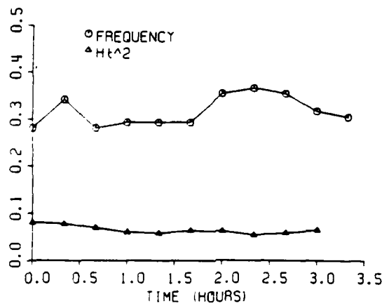
Fig. 31 — Temporal record of mean square wave height and peak frequency of wave spectrum for run 44.
