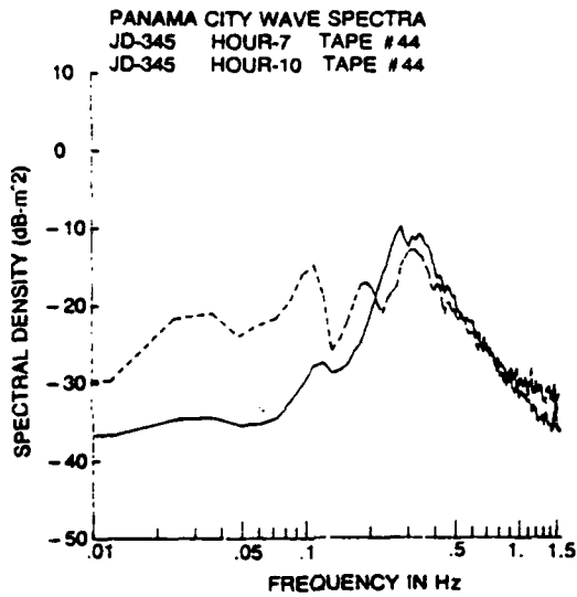
Fig. 30 — Change in spectral density between first and last hours of run 44.
