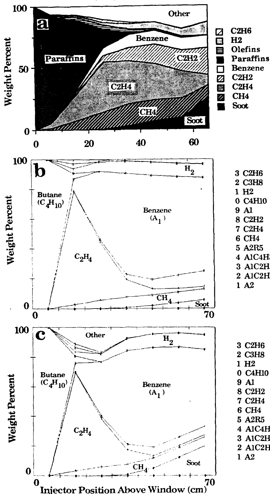
Figure 67. Comparison of Experiment with Simulations for Butane Pyrolysis at 1300°C as a Function of Reaction Distance. a) Experimental Data, b) Simulation with Rates of Table 9 and c) Simulation with Class Rate 21 Increased by Factor of 100.
