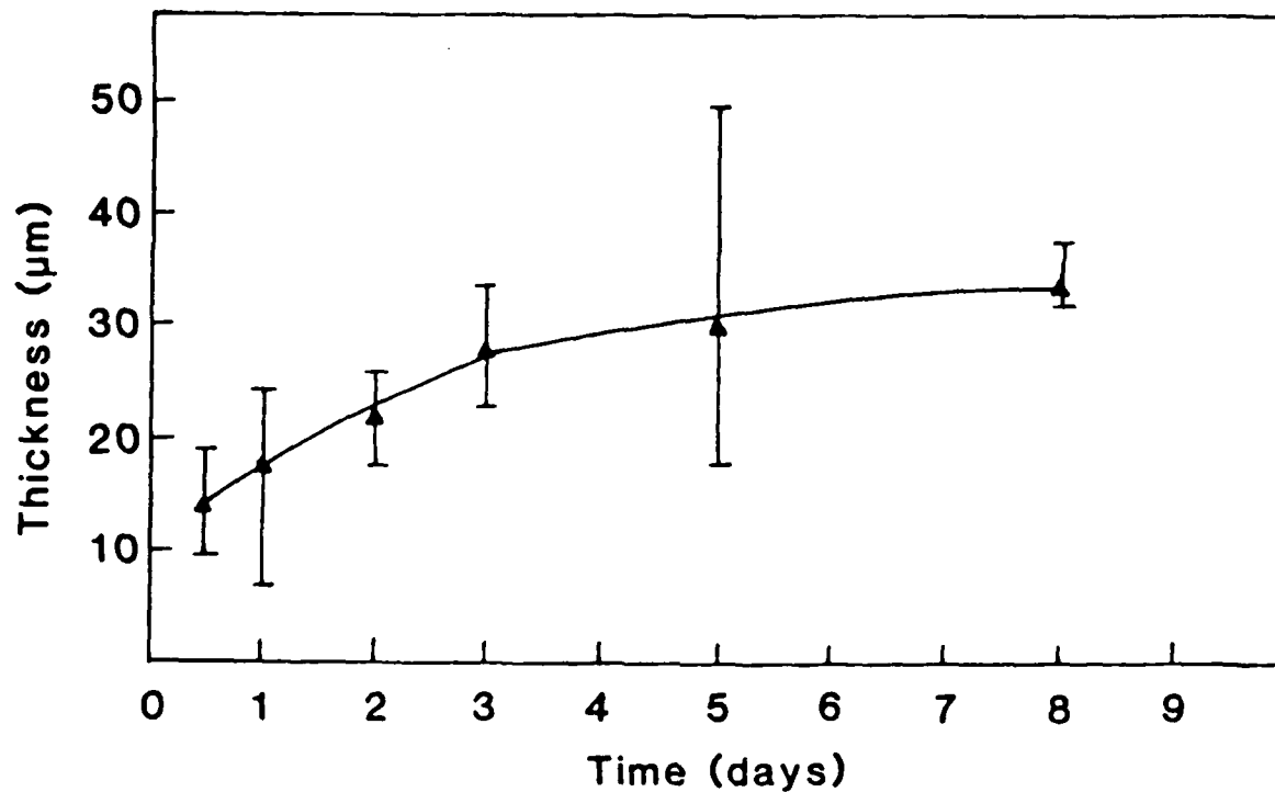
Fig.2 Thickness of the transform layer of stagnant samples versus corrosion time. ZBLA glass corroded in D.I. water, S/V:1.
