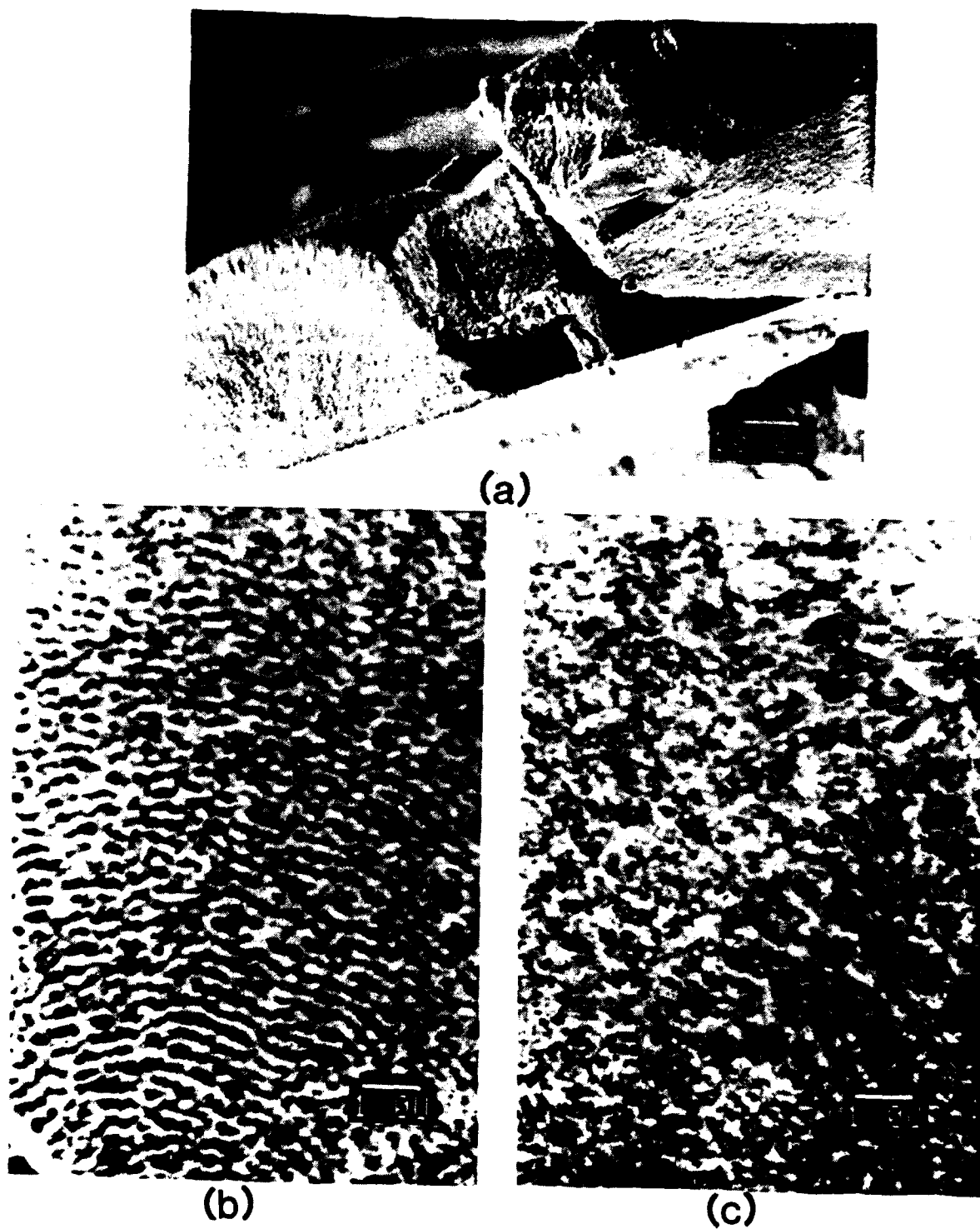
Figure 5.24. Cross-sectional view of precipitation layer formed on ZBLA glass after being corroded at S/V=1 for 7 days, (b) inner portion of the layer, (c) outer portion of the layer.
