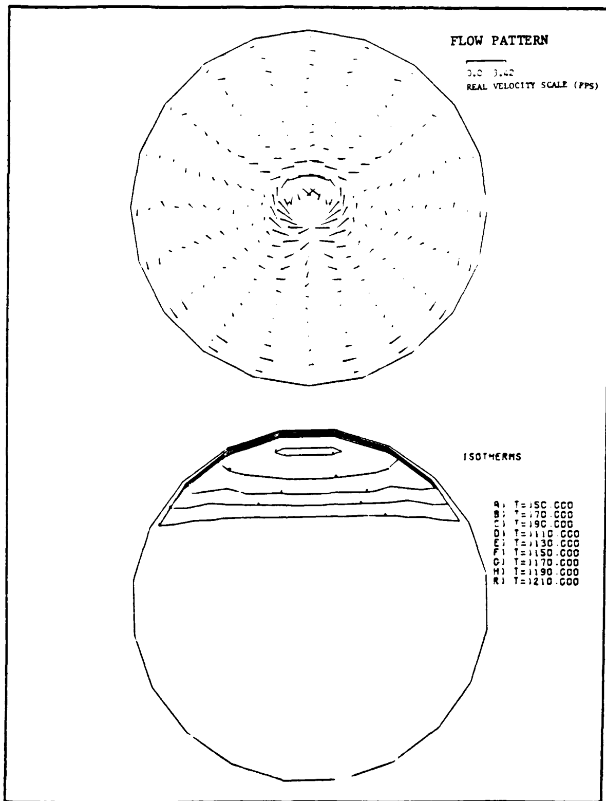
Figure 6.30 Velocity and Isotherm Plots after 130 Sec at the Thermocouple Rack
