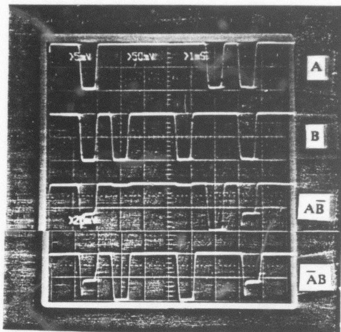
Figure 8. Experimental results of the inputs A, B and the logic outputs AB , \overline{AB} . The input powers are 11 mW each, and the output power is about 5 mW.
