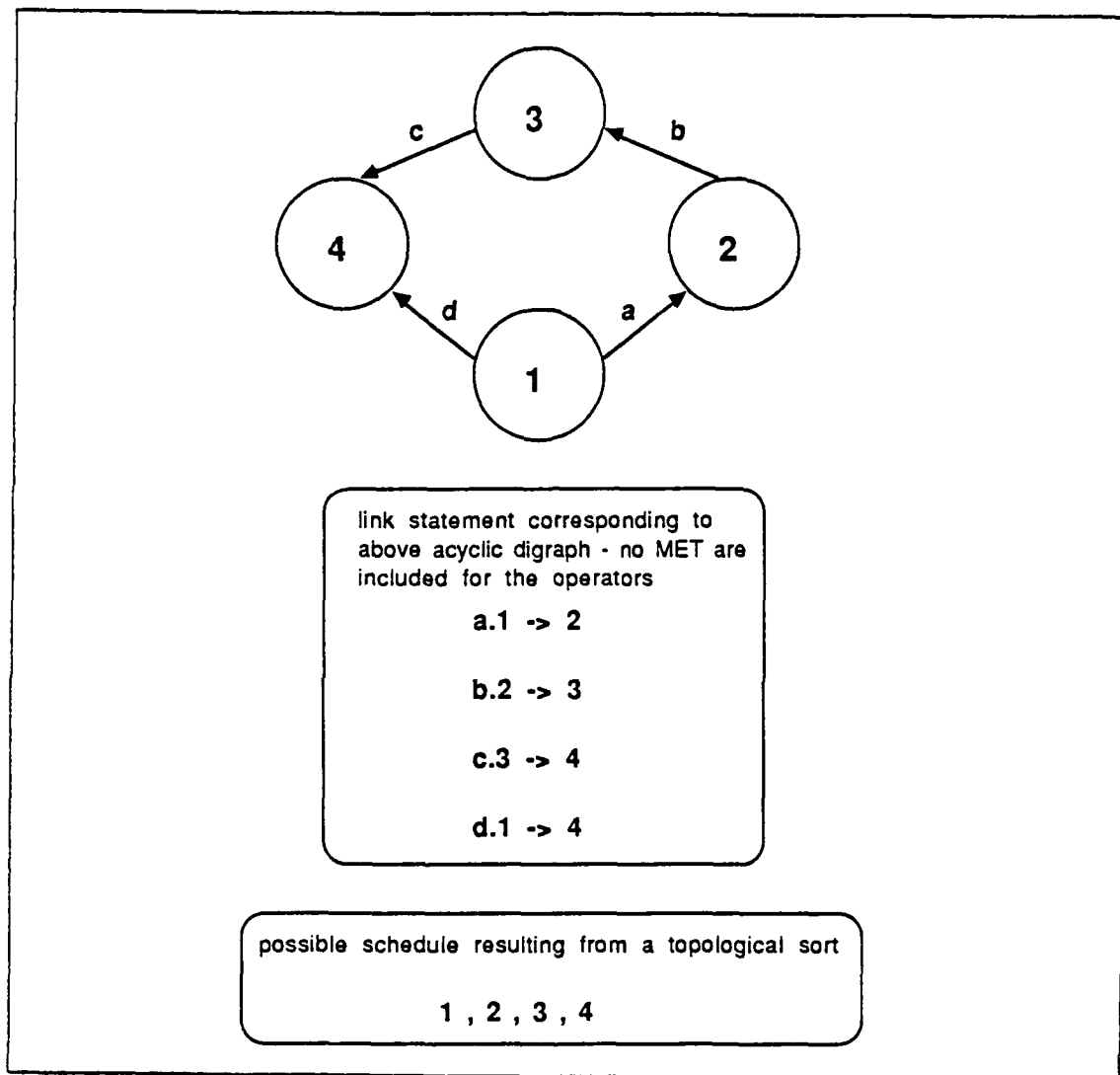
Figure 10. Acyclic Digraph
