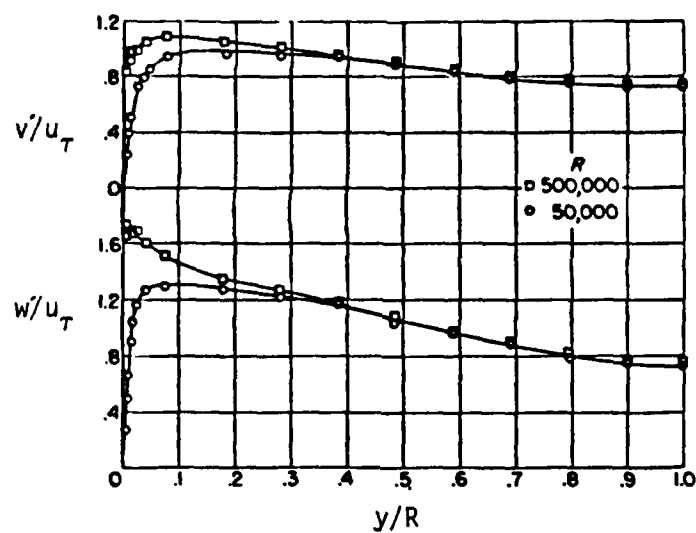
Figure 3.1 - Distribution of v'/u and w'/u
