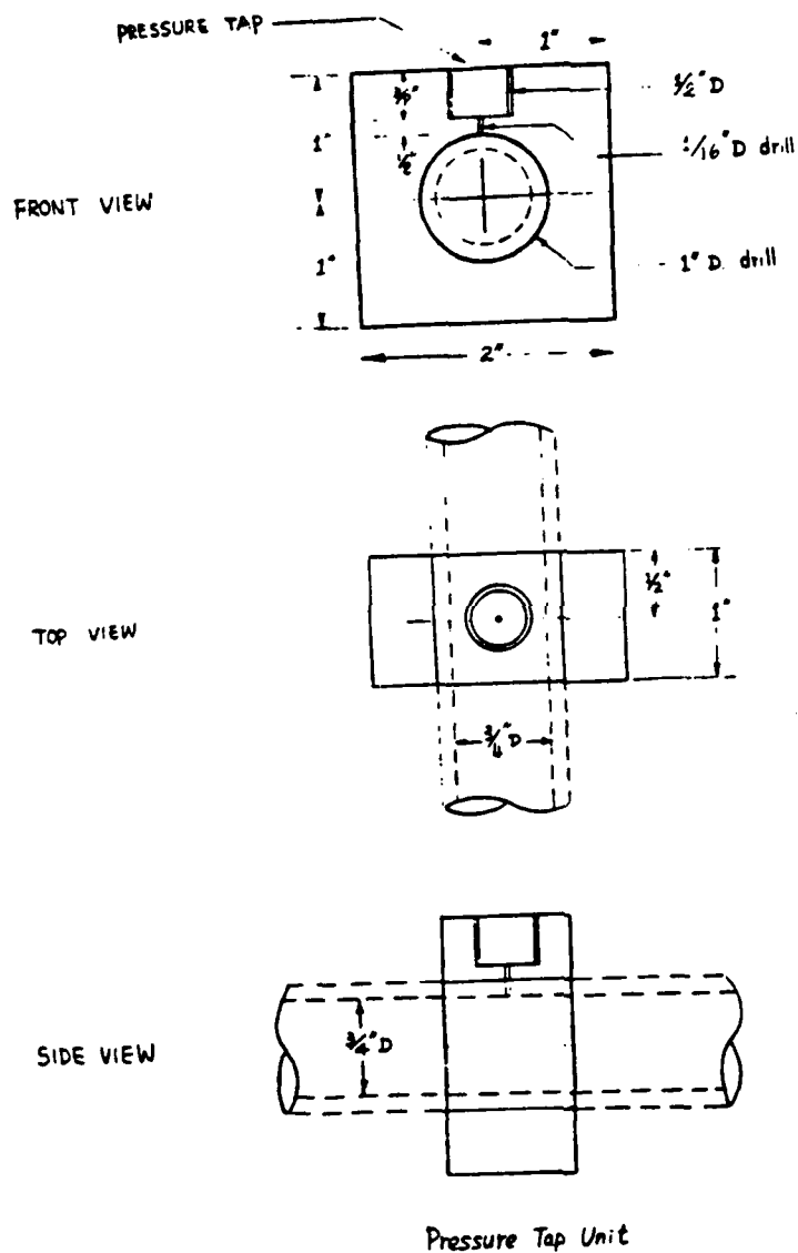
Figure 2.4 - Pressure Tap Configuration
