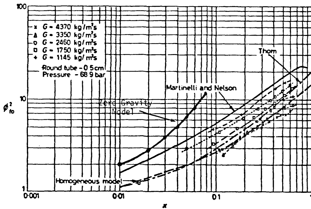
Figure 3.4 - Two-Phase Friction Multiplier for Steam-Water at 68.9 bar - Reproduced from Ref. 67
