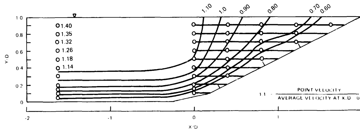
Figure 4.22. Velocity profiles, CSU Phase IV side slope tests
