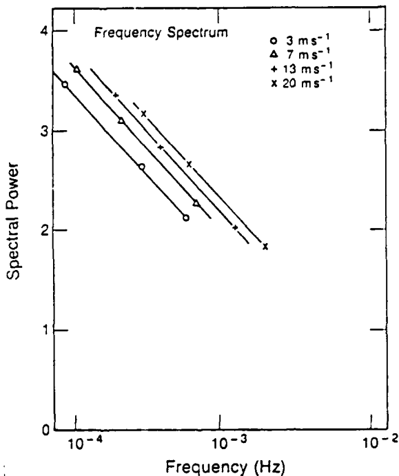
Fig. 4. Doppler shifted frequency spectra of horizontal velocity determined by Taylor transformation of the model wavenumber spectrum contained in Fig. 3.
