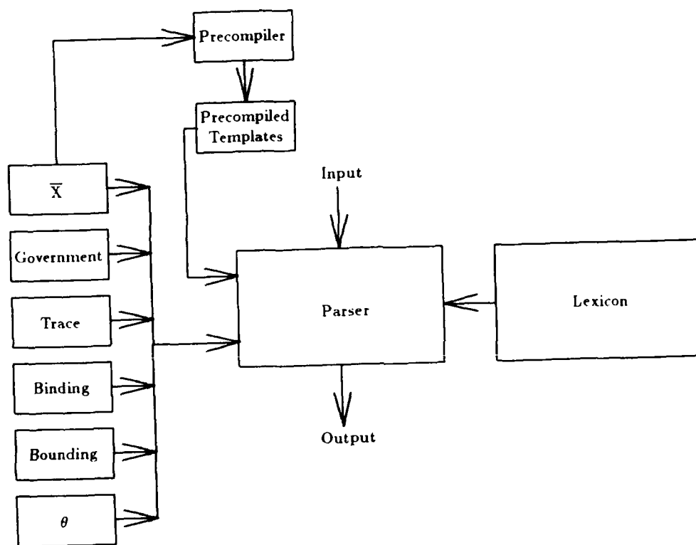
Figure 9.2: Lexically-Driven Parsing
