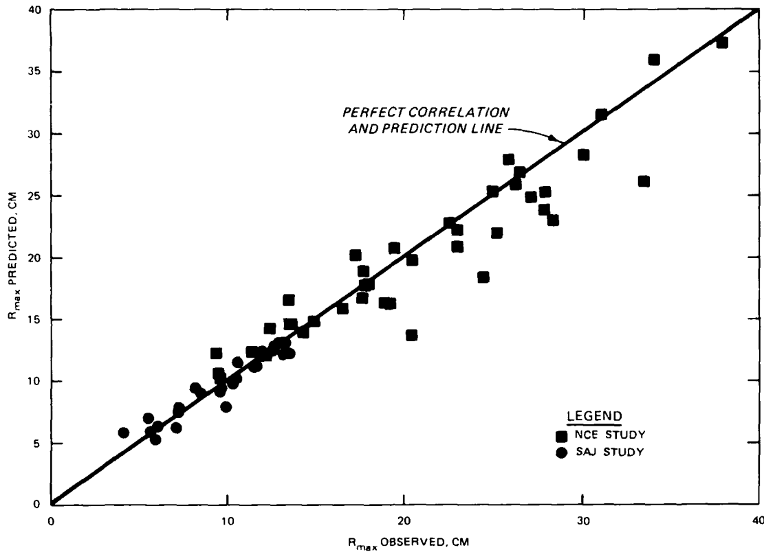
Figure 9. R_{max} predicted, using coefficients from both NCE and SAJ data, versus R_{max} observed for NCE and SAJ data
