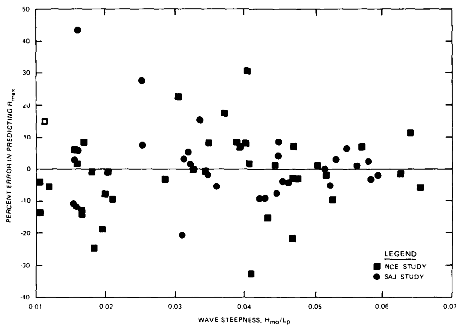
d. Percent error R_{max} versus steepness, H_{mo}/L_p
