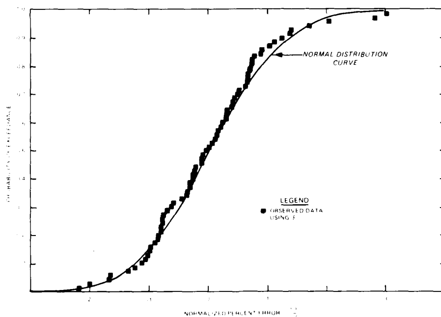
Figure 14. Normal distribution curve for \xi model data
