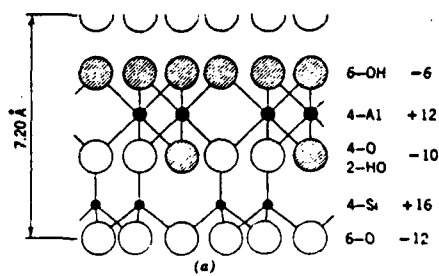
figure 5 The structure of kaolin (from Lambe and Whitman, 1979) a) atomic structure b) symbolic structure
