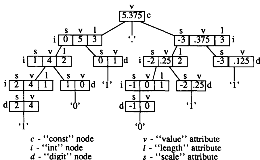
- Figure 1.3: Evaluated Structure Tree for Binary Number 101.011 -
