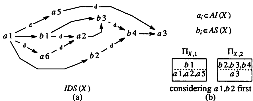
effectiveness of MAS() depends on which of the exclusive pairs is considered first - Figure 3.7 -
