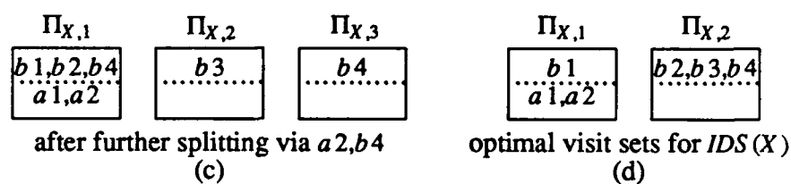
application of MAS() to IDS(X) having multiple instances of exclusive pairs - Figure 3.6 -
