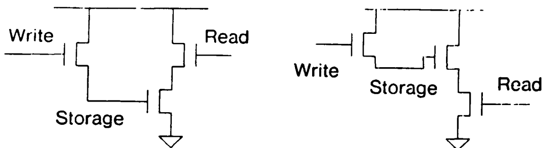
Figure 12.1: Two Three-Transistor RAMS
