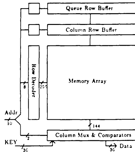
Figure 7: MDP Memory Block Diagram
