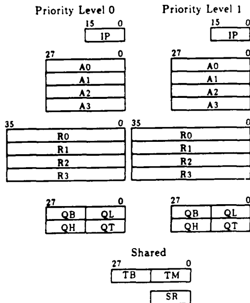
Figure 2: MDP Registers
