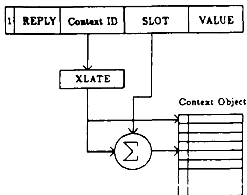
Figure 11: Processing A Reply Message
