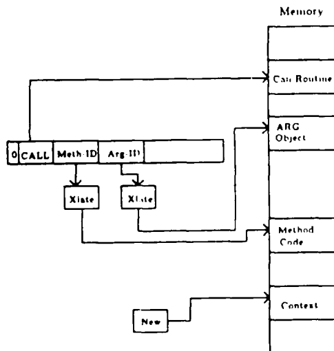
Figure 9: Processing a CALL Message
