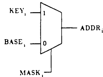
Figure 3: Translation Buffer Address Formation
