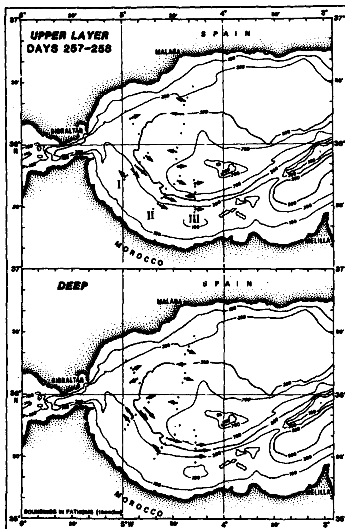
Fig. 47. Schematic results of geostrophic current calculations for the upper and deeper layers. CTD, cruise: Magnaghi, September 1982. Level of no-motion at 250 m. Roman numbers identify the cross-sections used for the calculation.
