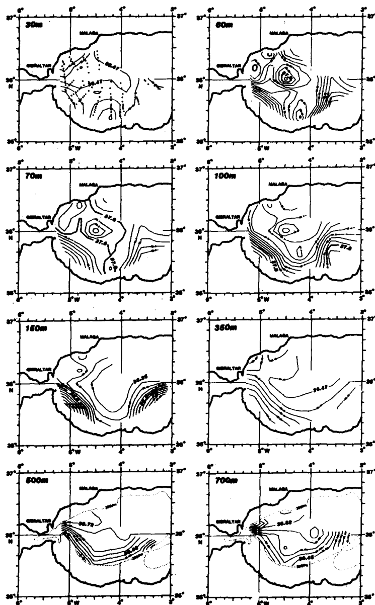
Fig. 41. Contours of salinity for the depths of 30, 60, 70, 100, 150, 350, 500 and 700 m. CTD, cruise: Alboran II, October 1983. Dots signify the positions of CTD casts.
