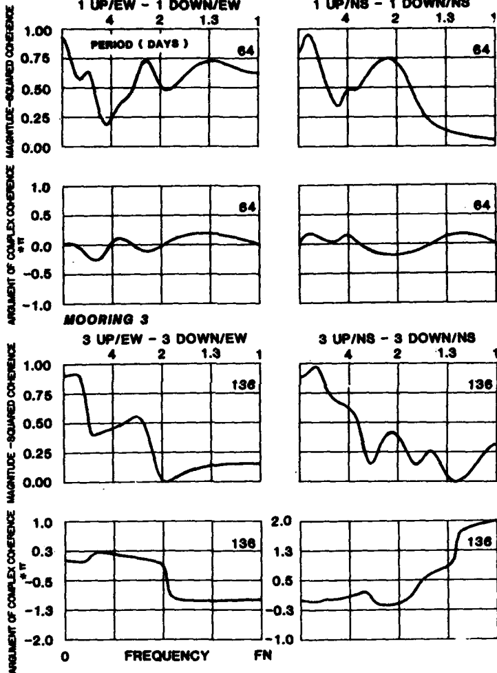
Fig. 6b. Magnitude-squared coherence and argument of complex coherence between the current velocity components measured by upper and lower current meters on each mooring. UP and DOWN signify the upper and lower current meters and EW and NS signify the east-west and the north-south current velocity components. Frequency scale is linear, FN marks the Nyquist frequency. Number on the right signifies the number of samples in the time series.
