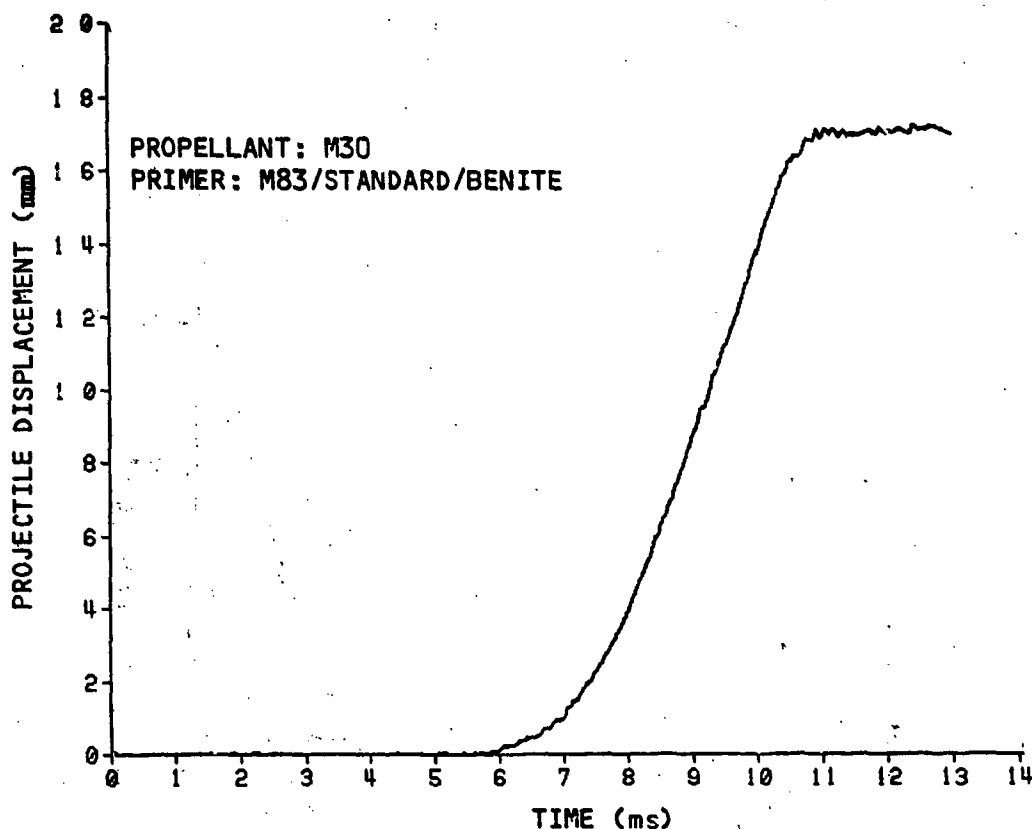
Figure 29. Typical Projectile Displacement.
