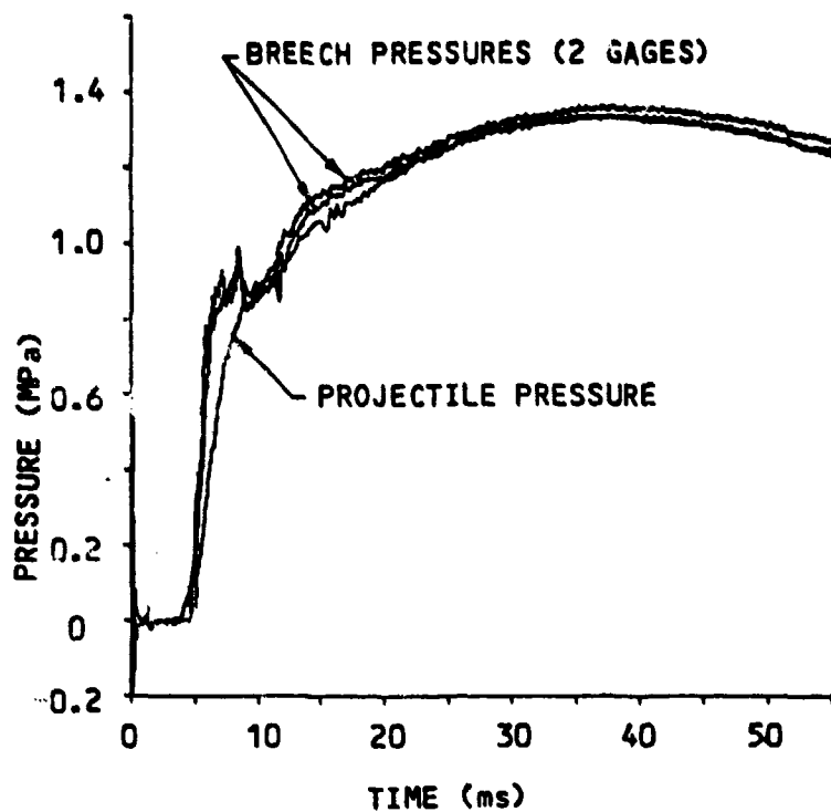
Figure 9. Pressures in an Inert Propellant Packed Chamber (Large Grains)
