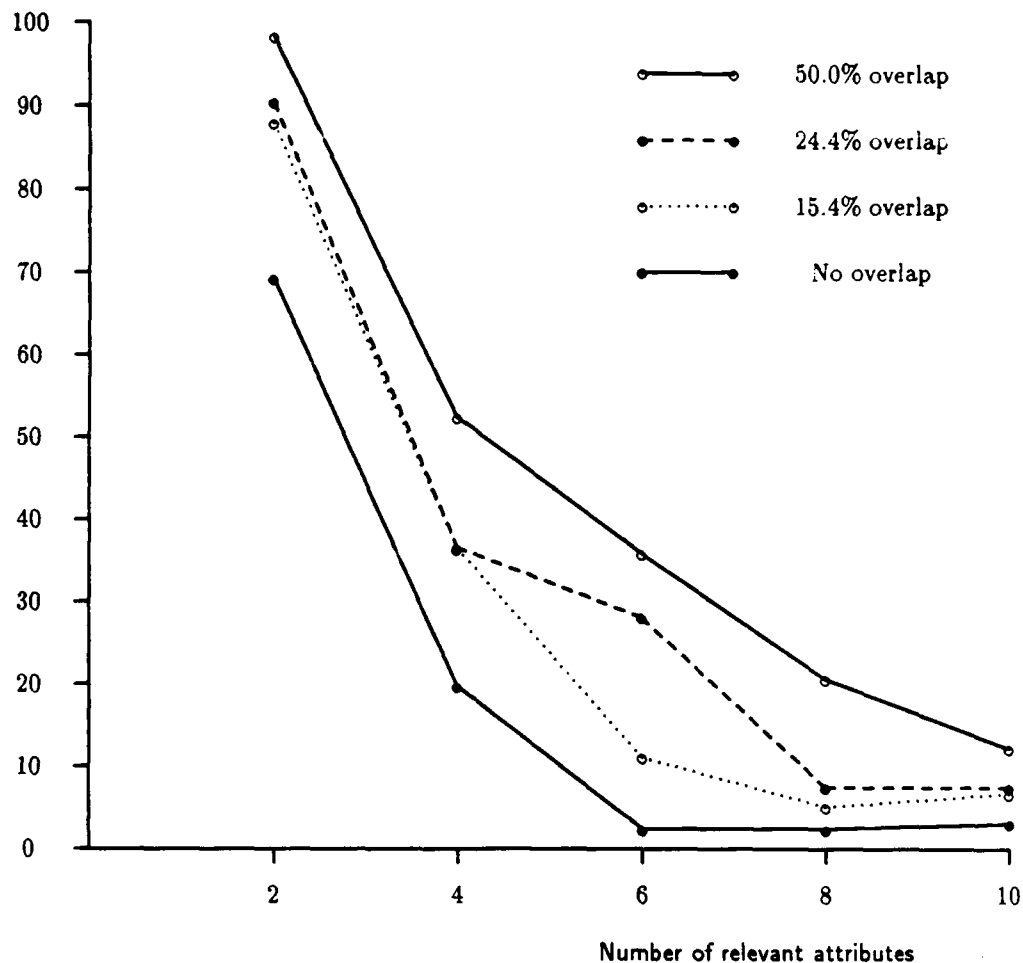
FIGURE 15. The effect of overlap and redundancy.
