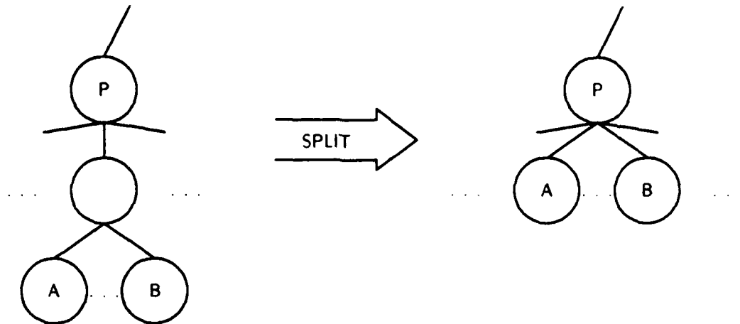
FIGURE 5. Splitting categories in COBWEB.
