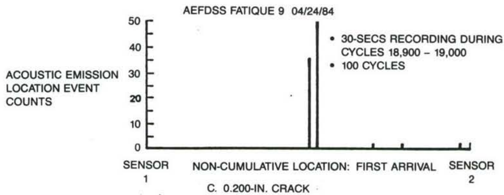
Fig. 18 Data for Specimen 9
