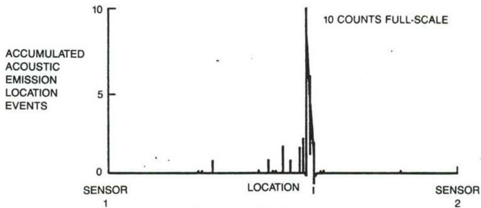
B. 0.050-IN. CRACK
