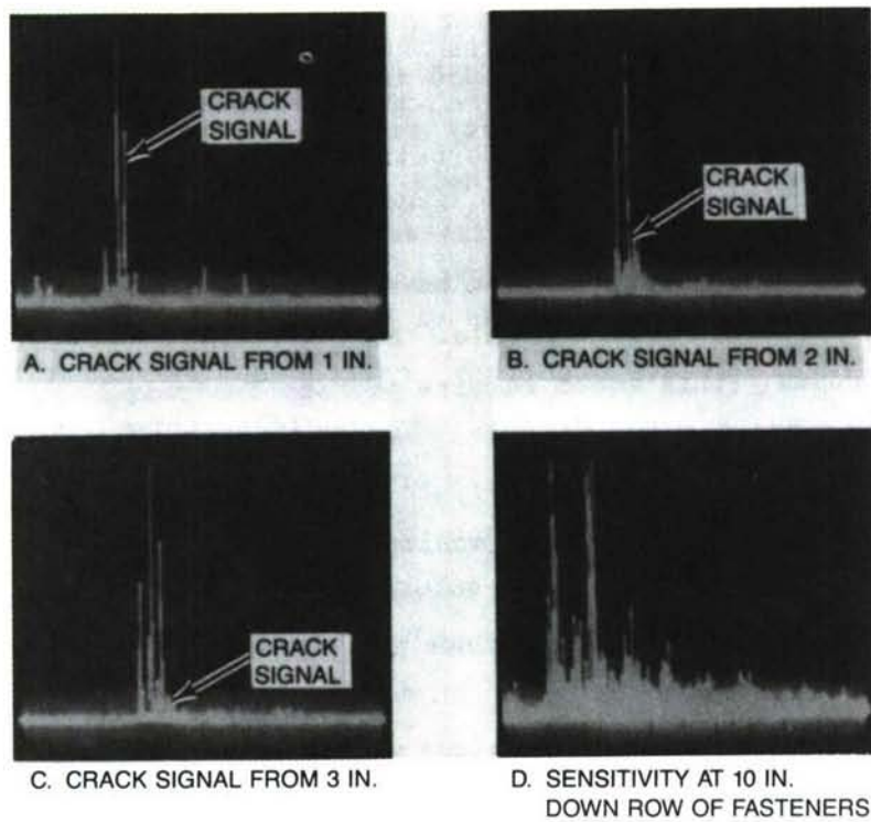
Fig. 2 Ultrasonic System Sensitivity
