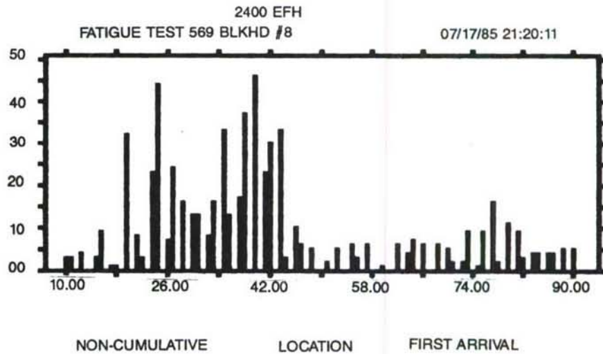
Fig. 34 Both Radii Showing Rapid Increase in Fatigue Damage
