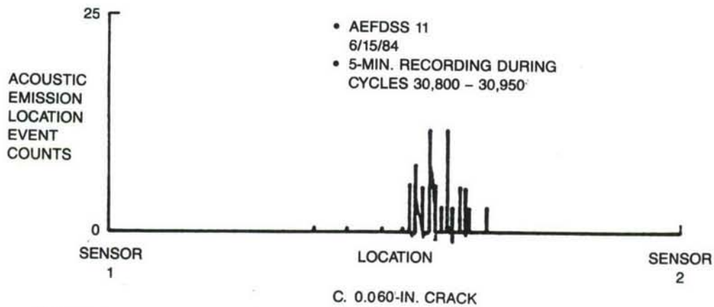
Fig. 20 Data for Specimen 11
