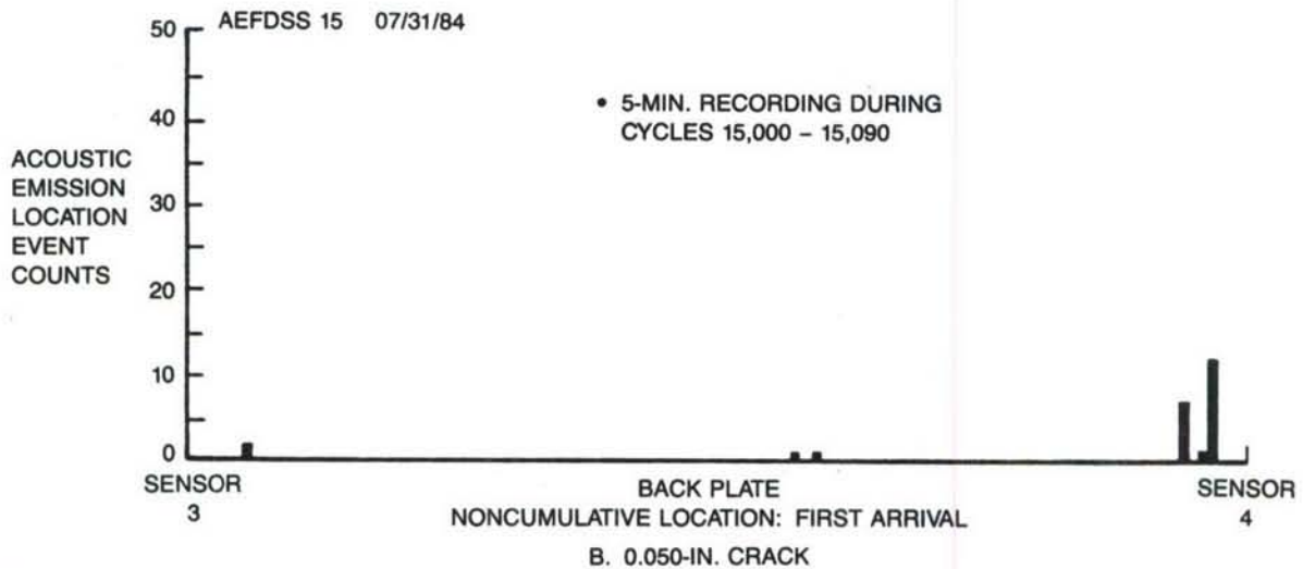
Fig. 25 Data for Specimen 15
