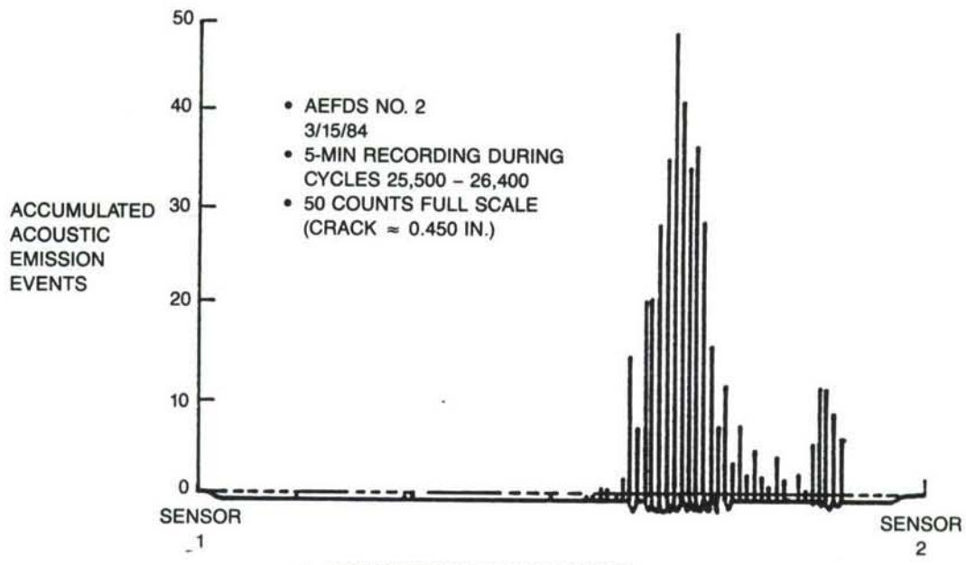
A. ACOUSTIC EMISSION LOCATION
