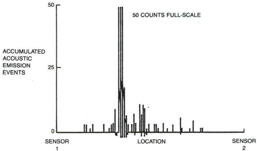
C. 0.100-IN. CRACK
