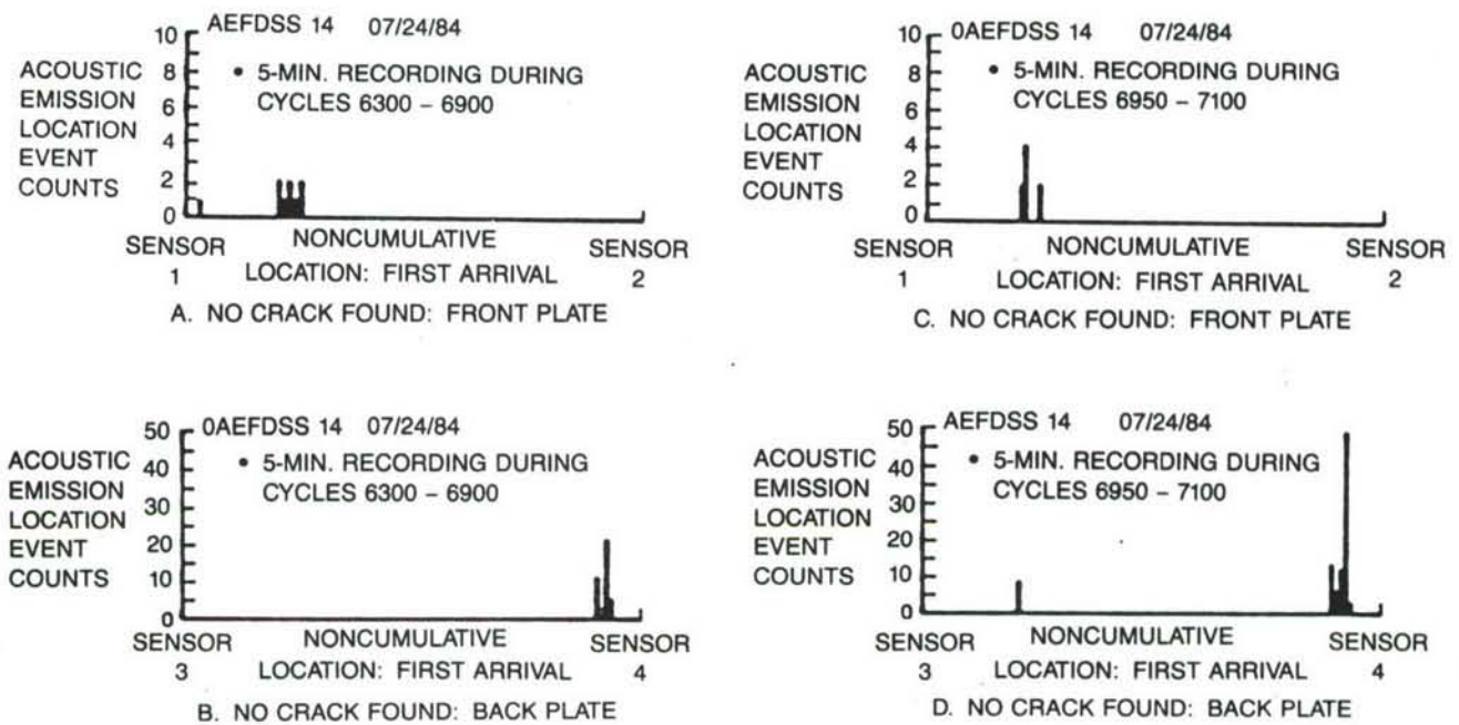
Fig. 22 Data for Specimen 14: Cycles 6300 to 7100
