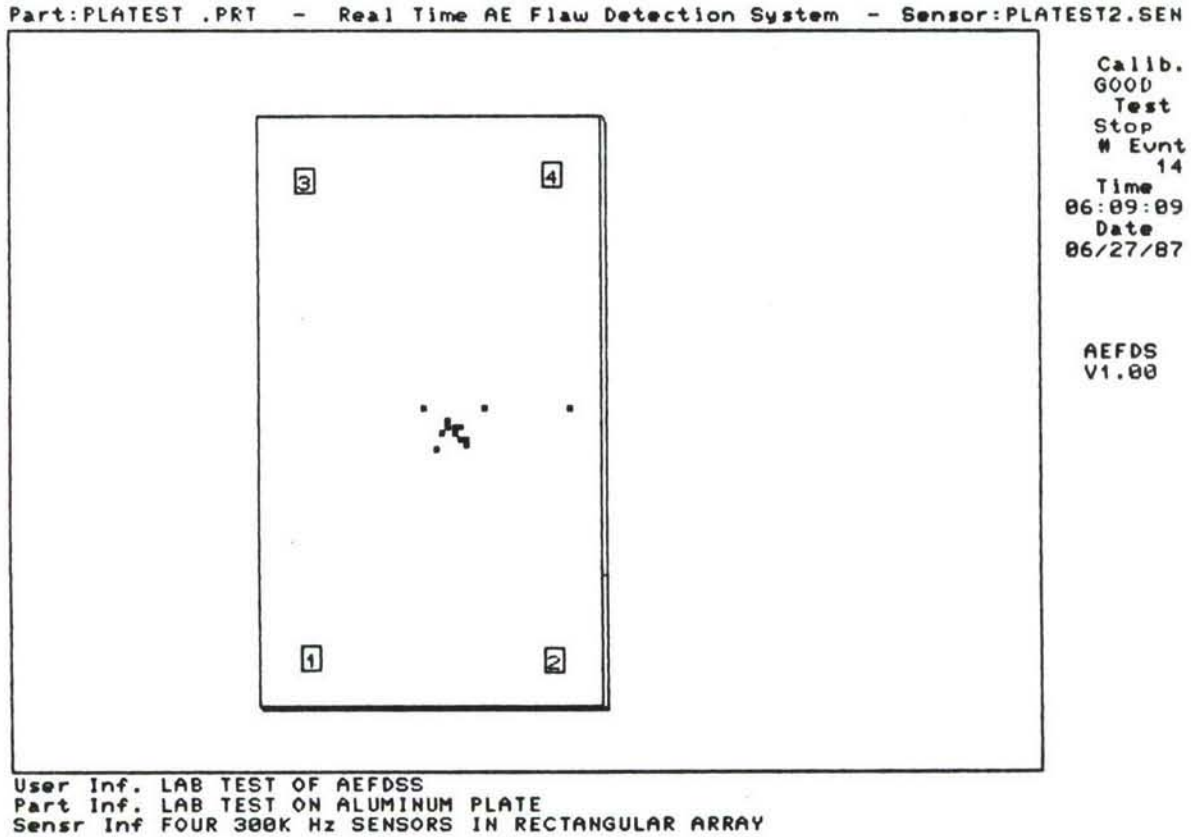
Fig. 41 Plots Obtained From 0.060-in. Crack
