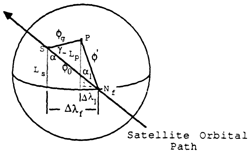
Figure 5. Satellite-Earth-Pixel Geometry
