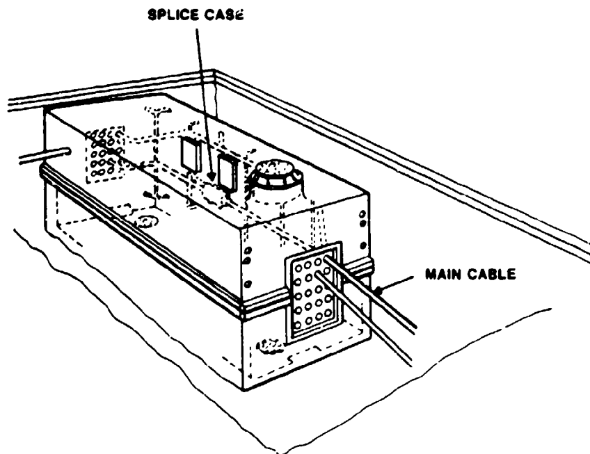
(b) Manhole-Installed Repeater
