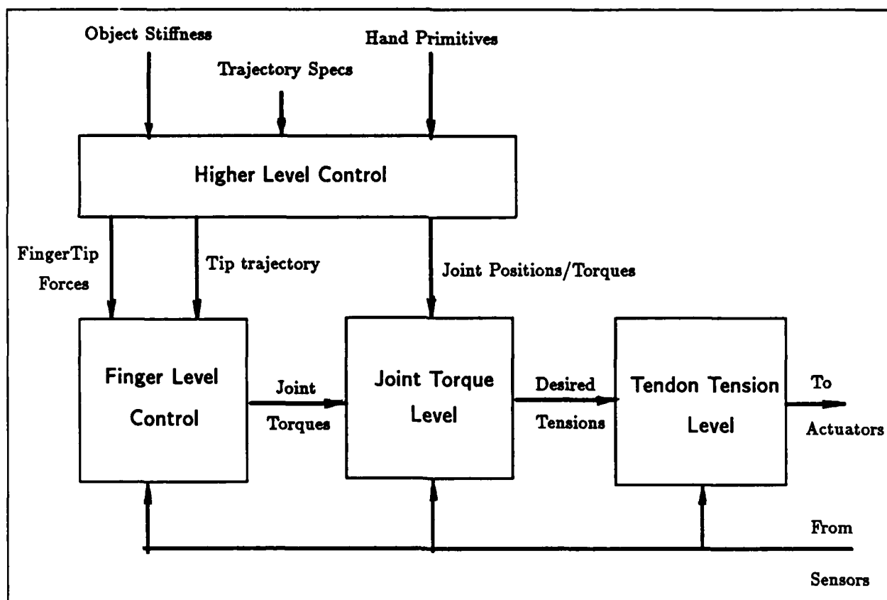
Figure 3: Block diagram of the controller
