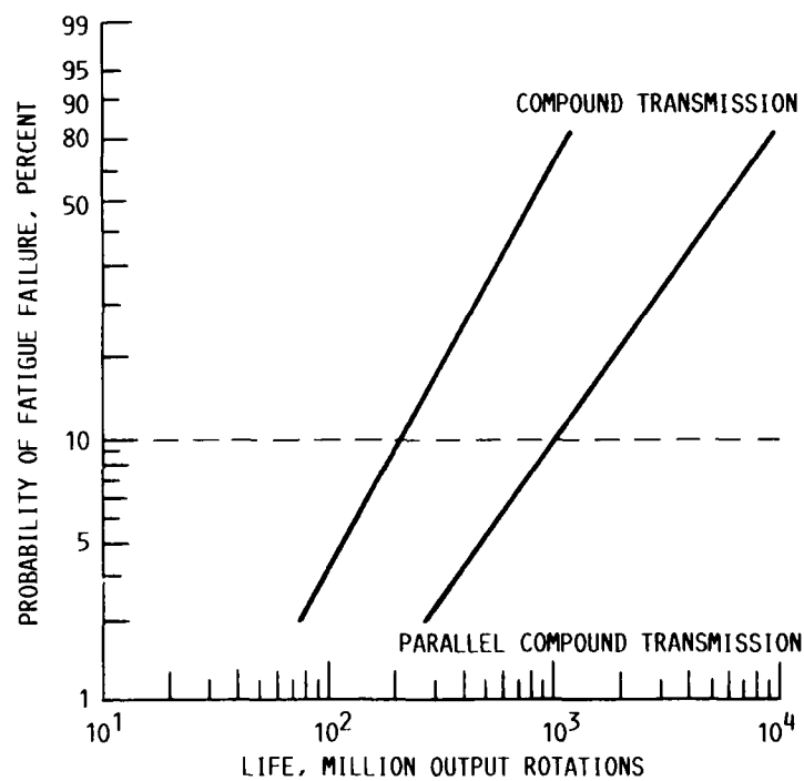
FIGURE 9. - EXAMPLE TRANSMISSION WEIBULL LIFE PLOTS.
