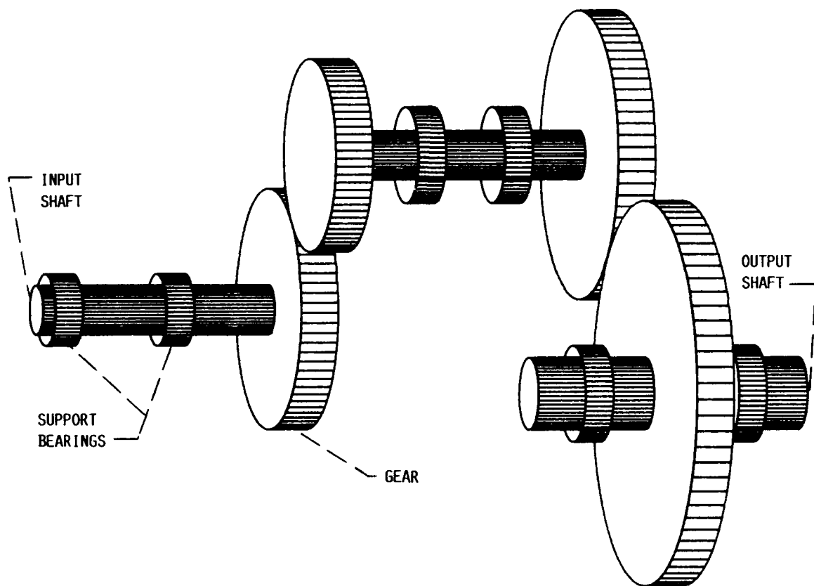
FIGURE 3. - COMPOUND GEAR TRANSMISSION.
