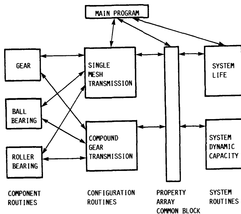
FIGURE 1. - PROGRAM STRUCTURE.
