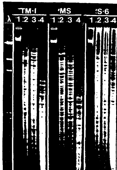
Figure 4. Agarose gel electrophoresis of whole and restriction enzyme-digested high molecular weight DNA from Methanosarcina thermophila TM-1, Methanosarcina barkeri MS, and Methanosarcina mazei S-6. Cultures were grown in marine medium, harvested by centrifugation and lysed with sodium dodecyl sulfate. Chromosomal DNA was purified by spooling precipitated DNA from ethanol. Lane \lambda is HindIII-digested lambda DNA included as a size standard. Lanes 1 through 4 are undigested (0.2 \mu g), AccI, EcoRI, and HaeIII-digested (10 \mu g) chromosomal DNA, respectively.
