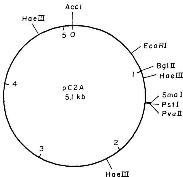
Figure 2. Map of plasmid pC2A from Methanosarcina acitivorans .
