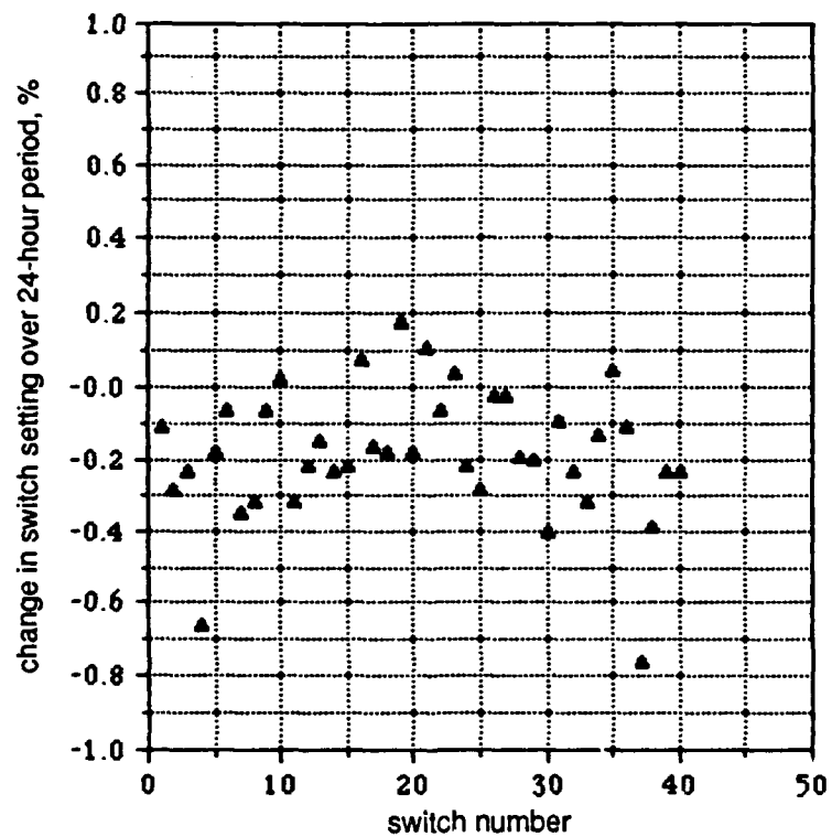
Figure 7. Data on accuracy and repeatability of the Custom Control Sensors pressure switch, PIN 607G6.
