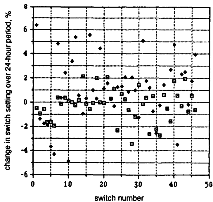
Figure 6. Data on accuracy and repeatability of the Whitman Controls pressure switch, P/N 1190.
