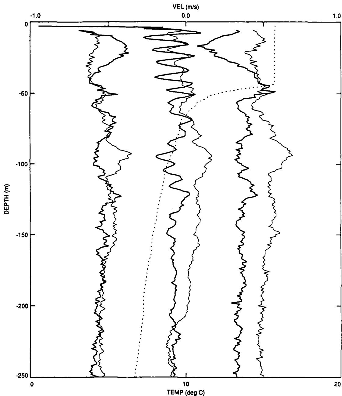
Figure 21. Plot of east (heavy line) and north (light line) velocities for slowfall AXCP 2202 (center) and regular AXCPs 2201 and 2203 (left and right). The three were deployed within a 4 s interval on 23 October 1987. The temperature profile ( ... ) obtained from the slowfall unit is overlaid. No gain or phase corrections have been made on the slowfall profile.
