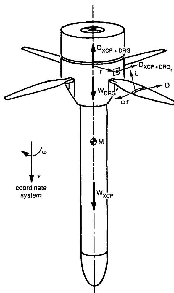
Figure 8. Two-dimensional, free-body diagram of the translational forces and rotational moments acting on the probe and drogue.
