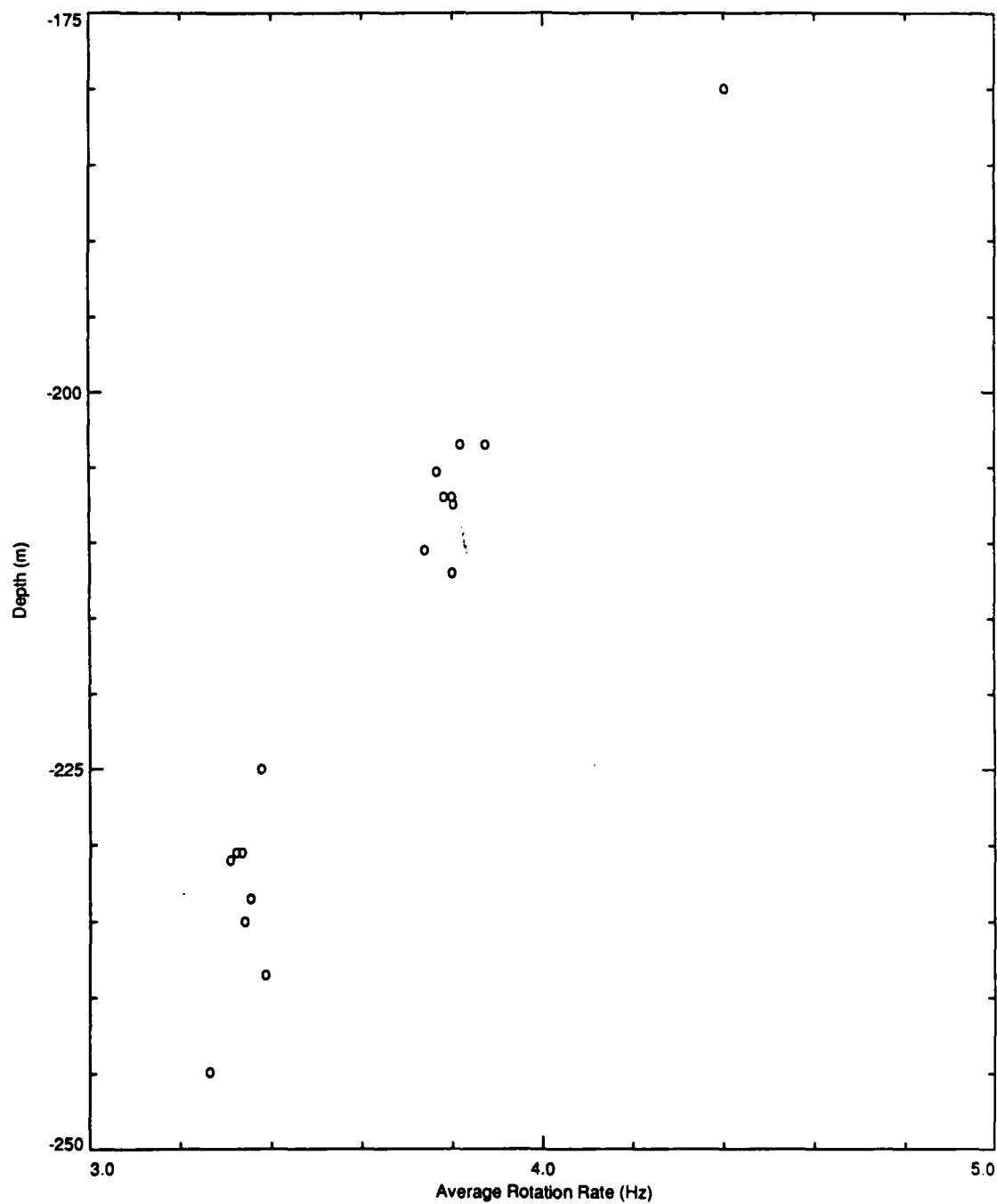
Figure 22. Squib fire depth versus average rotation rate for slowfall AXCPs. A fall rate of 0.72 \text{ m s}^{-1} is assumed for all probes in order to calculate apparent depths.
