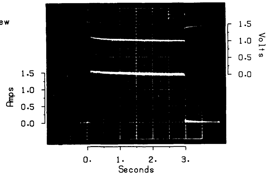
Figure 5. High current pulse output from alkaline AA and AAA cells.
