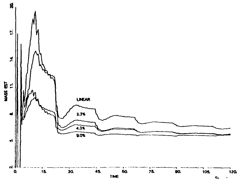
Figure 5.2: Effect of the Gap Nonlinearity on the Convergence of the Mass Estimates.
