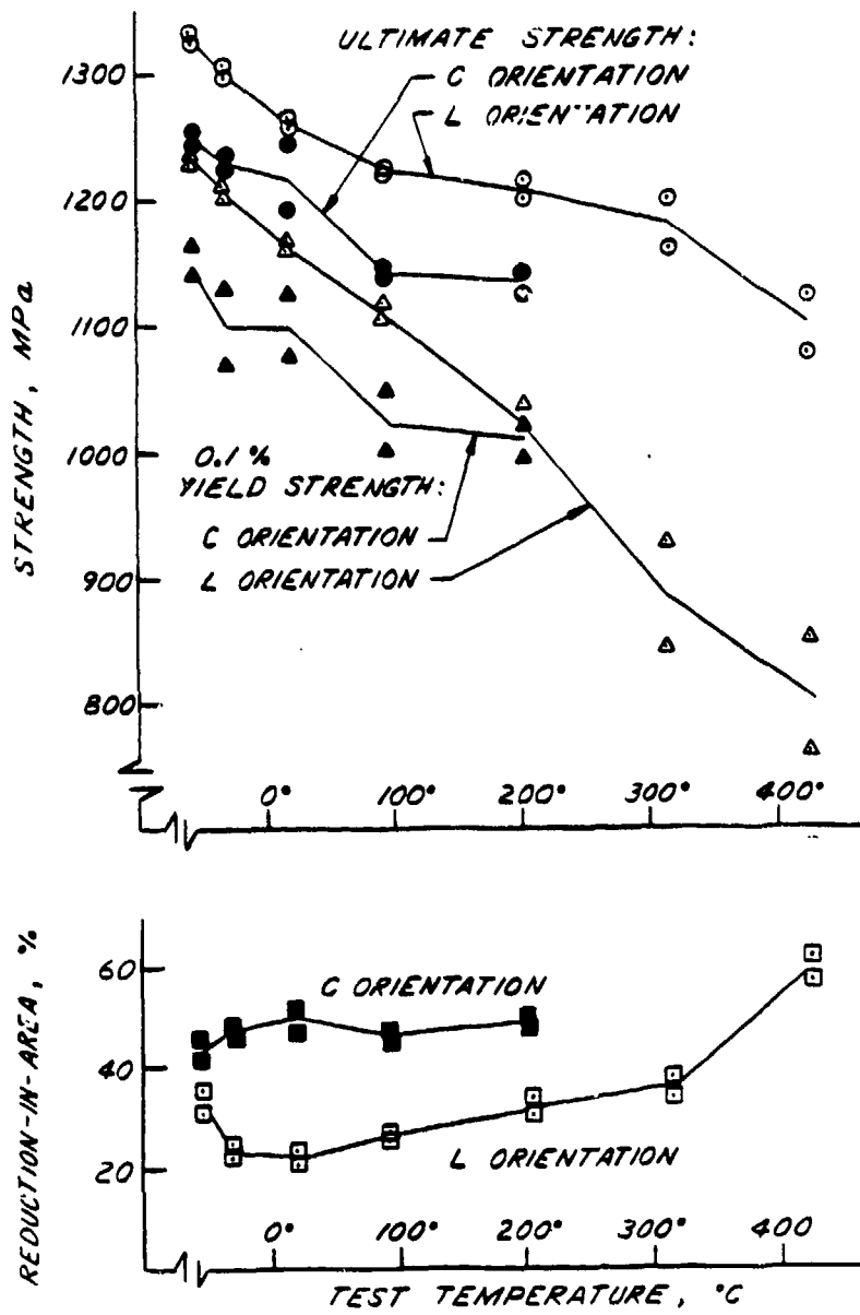
Figure 6. Effect of temperature on tensile mechanical properties of steel.
