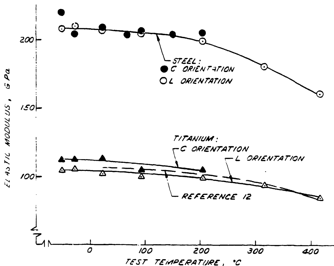
Figure 4. Effect of temperature on elastic modulus for steel and titanium.
