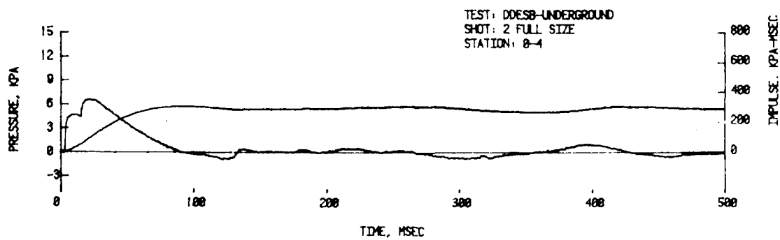
FIGURE B2. Predicted Full Scale Impulse for 9^{\circ} line, 1.101 \text{ kg/m}^3 , \sqrt{V} .
