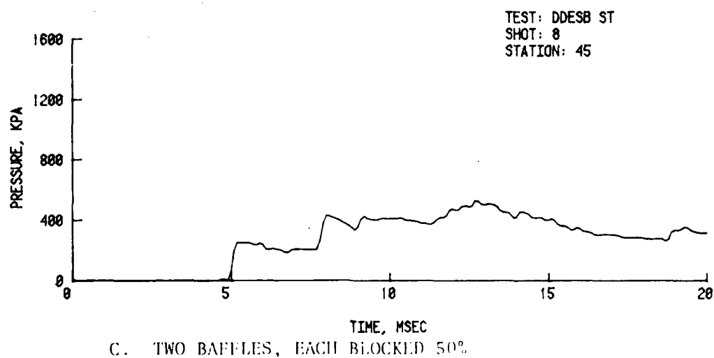
FIGURE 12. Attenuation Over 45 Test Section Diameters, Average Driver Pressure 814 kPa
