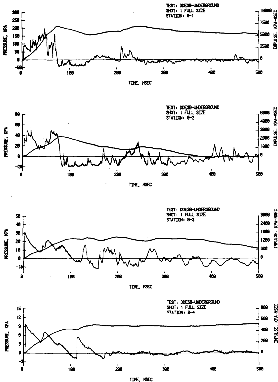
FIGURE B1. Predicted Full Scale Impulse for 0^{\circ} Line, 0.356 \text{ kg/m}^3 , q/v_c
