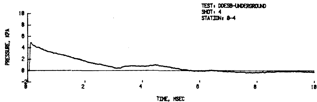
FIGURE A3. Shot 4, Chamber Loading Density - 3.405 \text{ kg/m}^3 of PRIMACORD (Cont)
