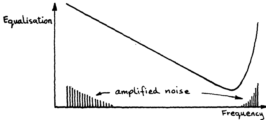
Fig 12 Typical record/replay response
