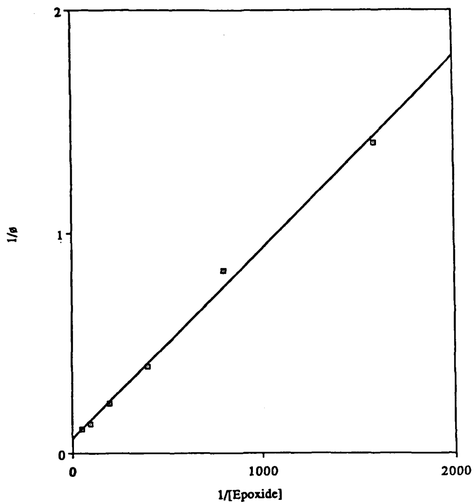
Figure 2. Double reciprocal plot of photooxygenation quantum yield vs. epoxide concentration for 7b in acetonitrile ( \phi_{lim} = 15.2 , r = 0.997 ).
