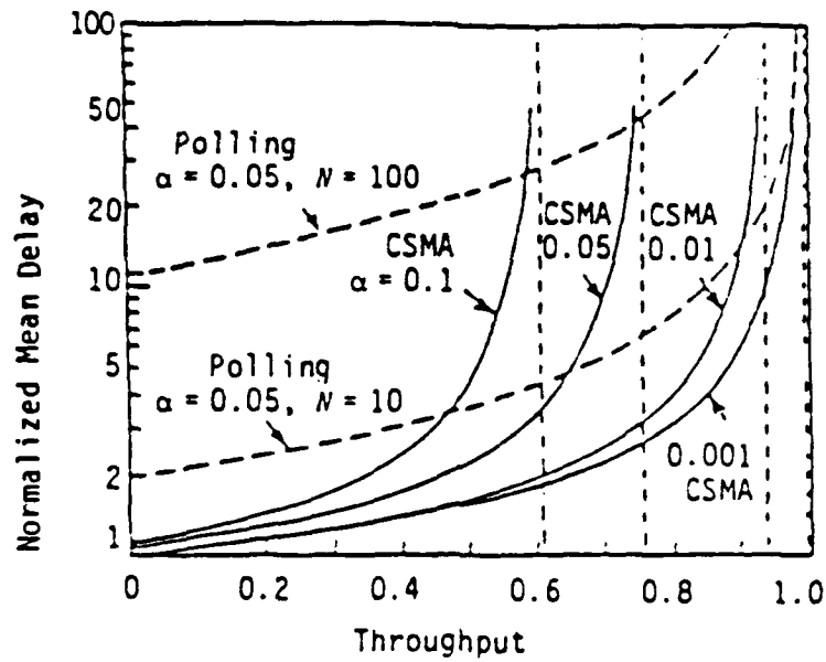
Figure 4-6. Mean Delay vs. Throughput: Polling and CSMA/CD.
