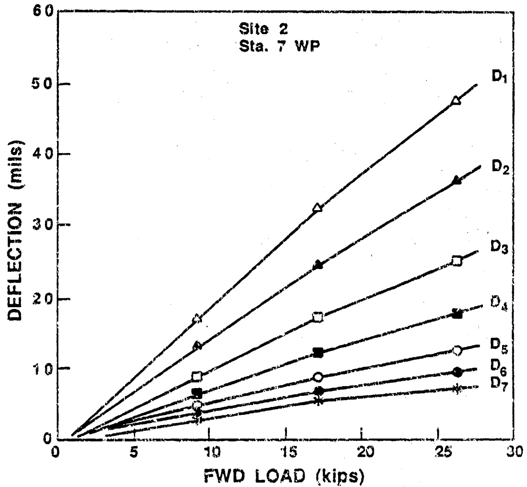
Figure 6.11 Surface Deflection as a Function of Load at Site 2 (Most Linear Response)
