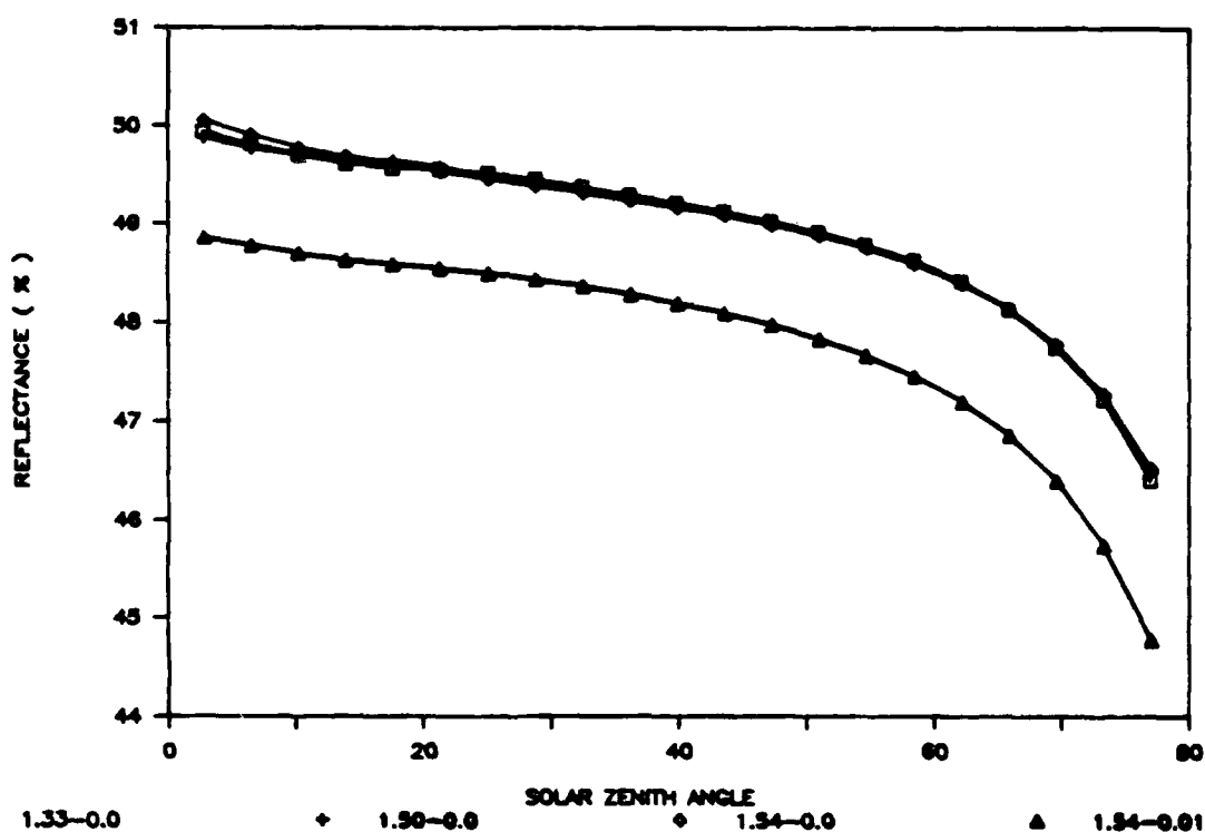
Figure 5.1 Comparison of the Effect of Varying the Aerosol Index of Refraction on Apparent Reflectance
